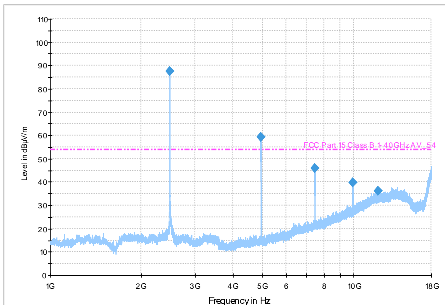
High Channel - Radiated Spurious Emissions 1 – 18GHz
