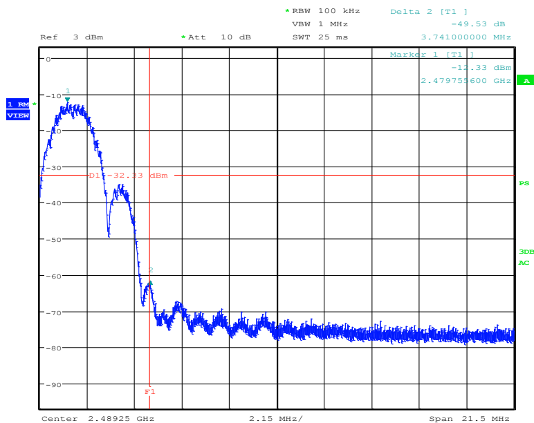
OUT OF BAND EMISSIONS - HIGH CHANNEL
