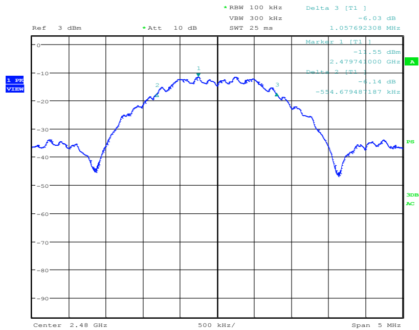
HIGH CHANNEL – 6dB OCCUPIED BANDWIDTH
