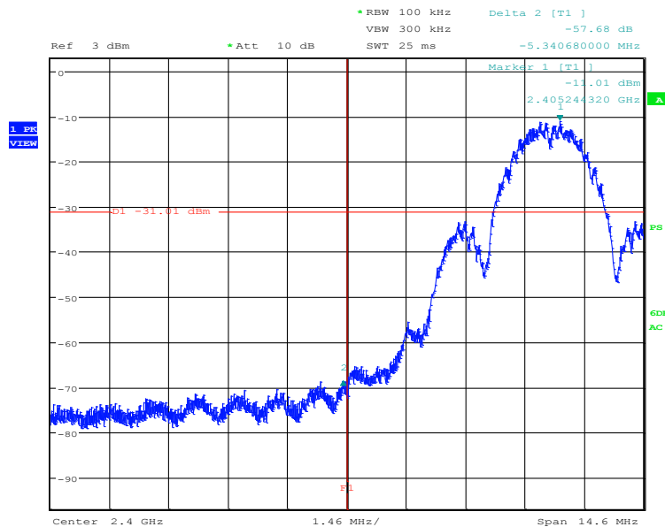
OUT OF BAND EMISSIONS - LOW CHANNEL
