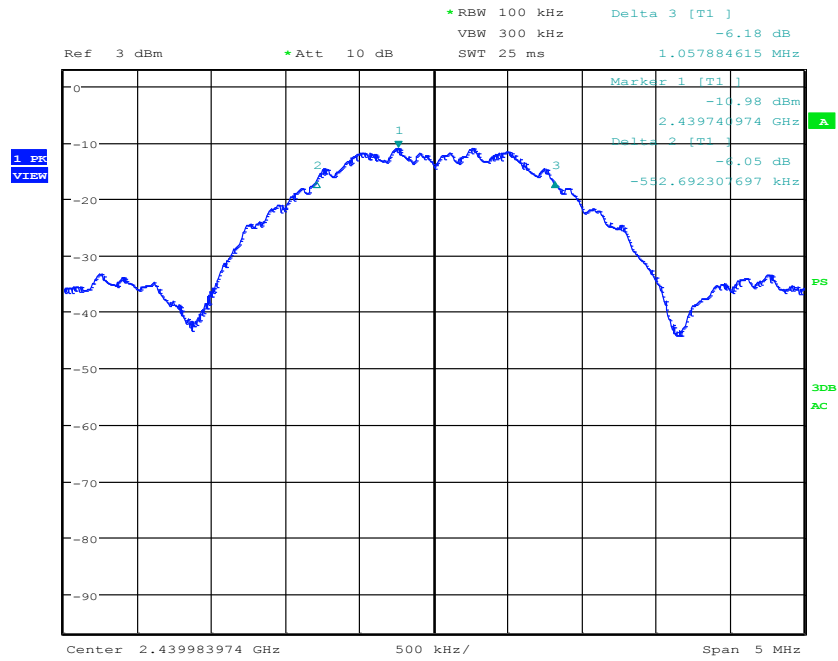
MID CHANNEL – 6dB OCCUPIED BANDWIDTH
