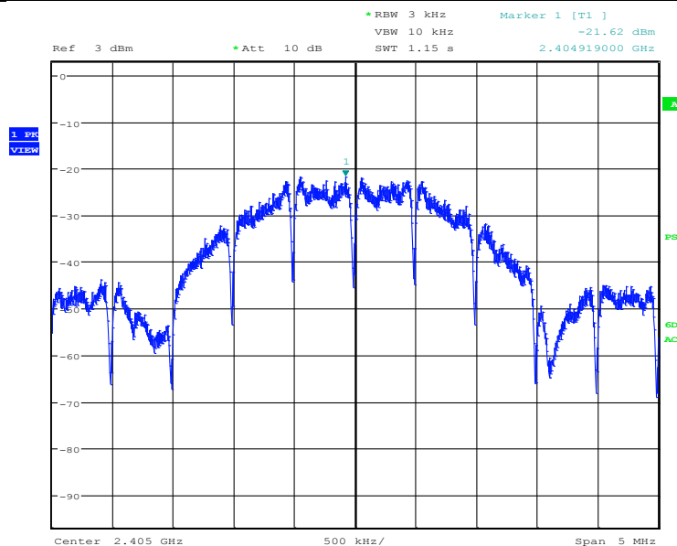
LOW CHANNEL - POWER SPECTRAL DENSITY
