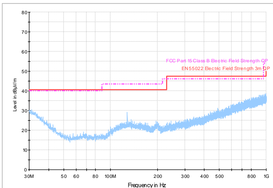
Low Channel Radiated Spurious Emissions 30MHz – 1GHz
