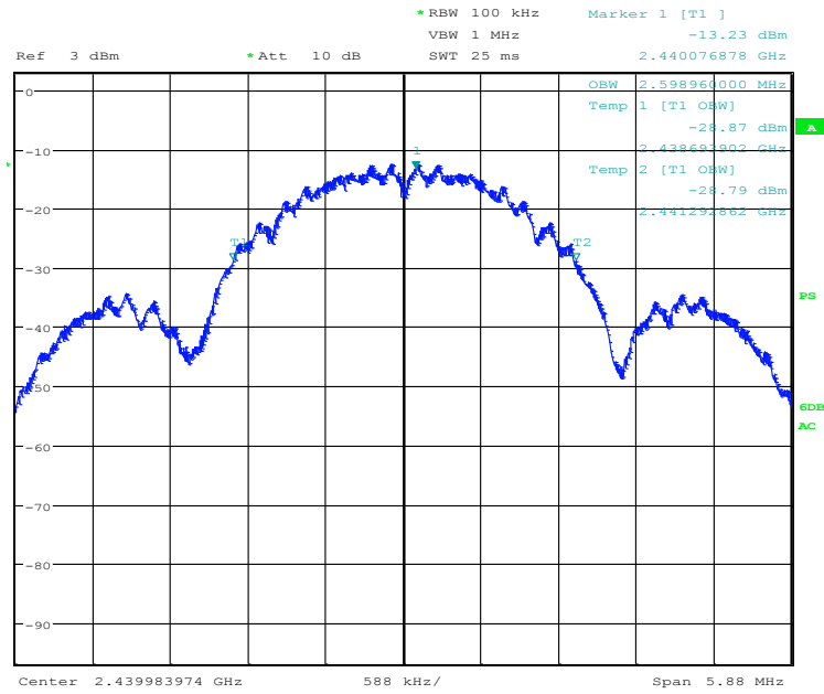
MIDDLE CHANNEL – 99% OCCUPIED BANDWIDTH
