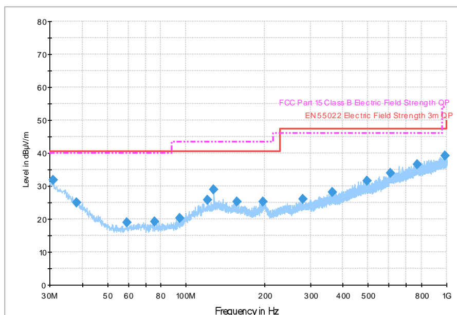
Radiated Emissions 30MHz – 1GHz, No-TX
