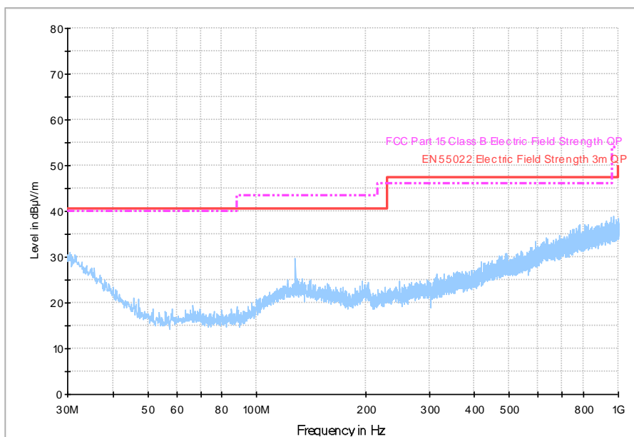
Middle Channel - Radiated Spurious Emissions 30MHz – 1GHz
