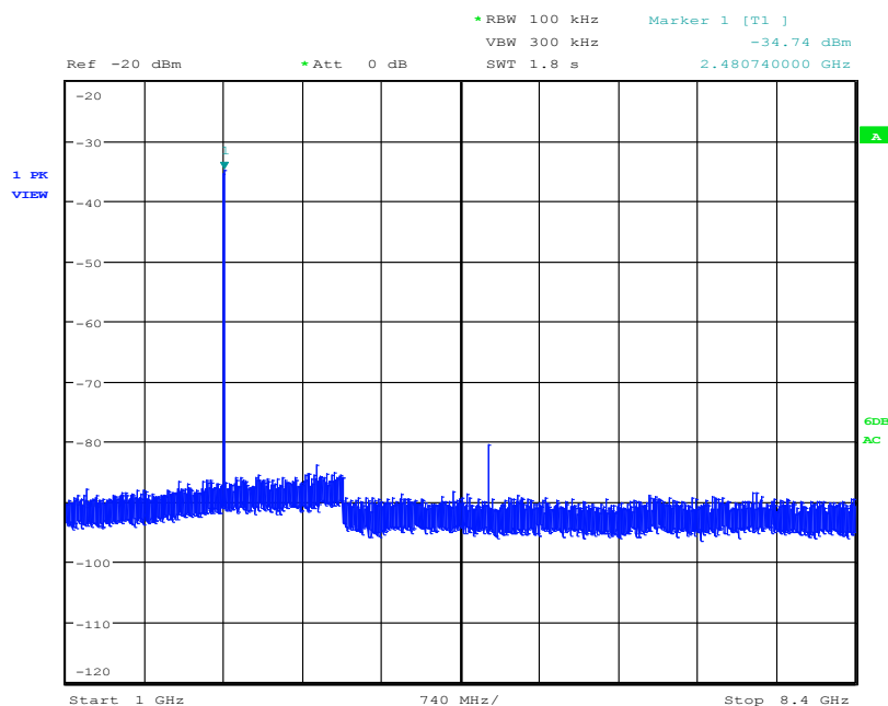
High Channel - Conducted Spurious Emissions 1 – 8.4GHz
