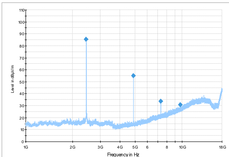
Middle Channel - Radiated Spurious Emissions 1-18GHz
