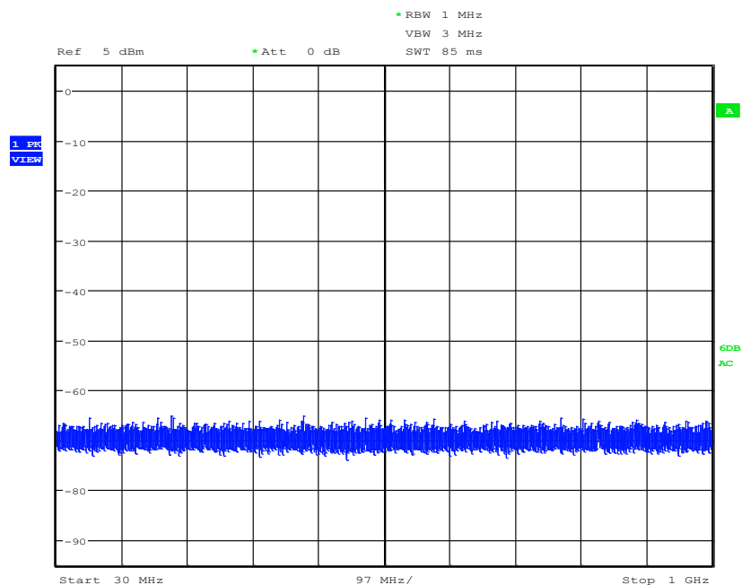
Middle Channel - Conducted Spurious Emissions 30MHz-1G
