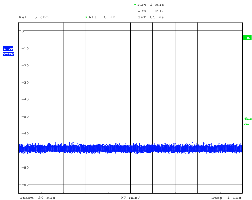
High Channel - Conducted Spurious Emissions 30MHz-1GHz
