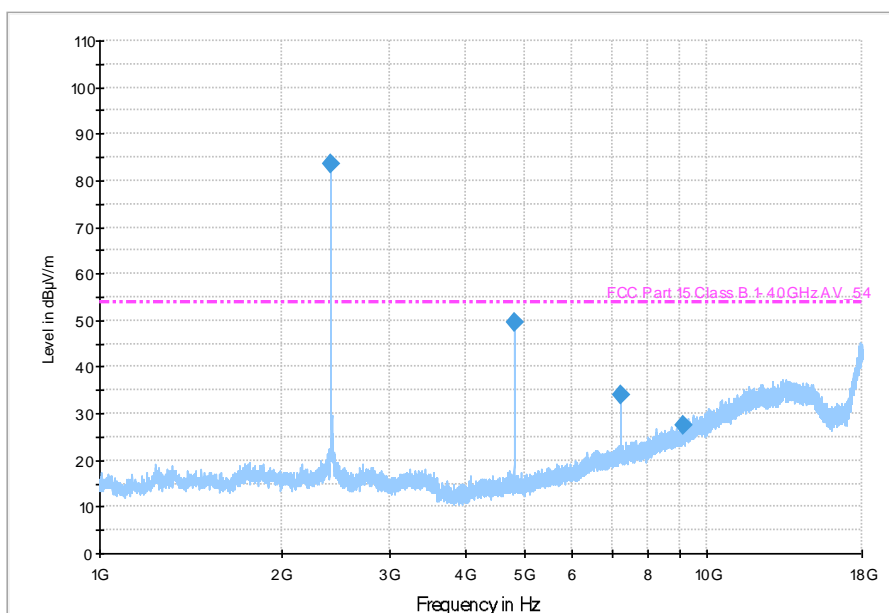
Low Channel Radiated Spurious Emissions 1 – 18GHz
