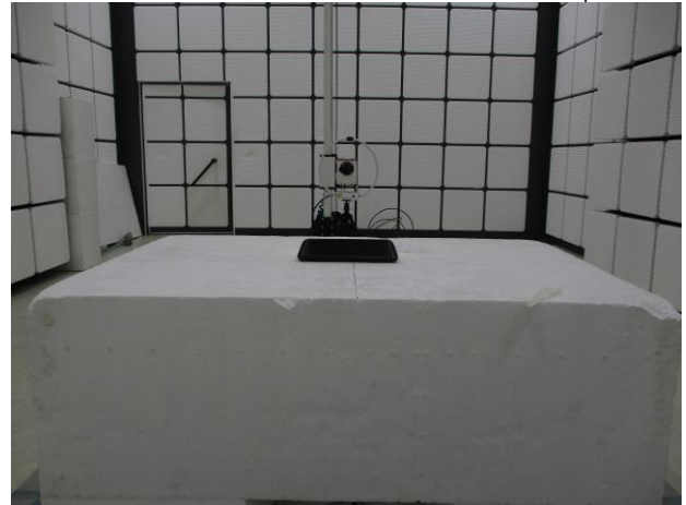
FCC_15_247_902~928MHz_LoRa_Radiated_Setup
