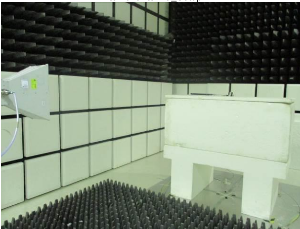
FCC_15_247+IC_RSS_247_902~928MHz_LoRa_Radiated_ Internal antenna_Setup
