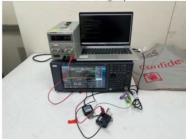
FCC_15_247+IC_RSS_247_902~928MHz_FSK_Radiated_ Internal antenna_Setup
