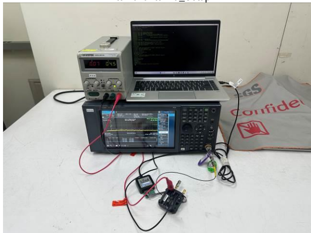
FCC_15_247+IC_RSS_247_902~928MHz_LoRa_Conducted_ Internal antenna_Setup
