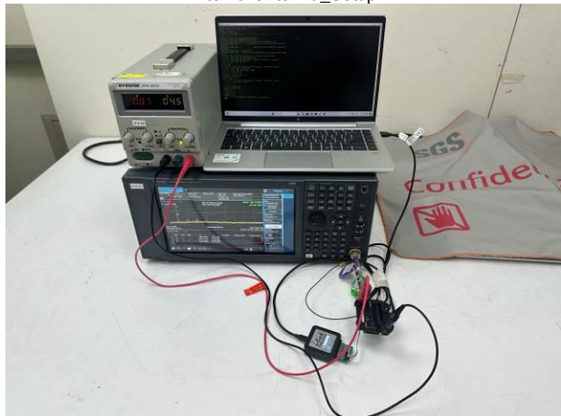
FCC_15_247+IC_RSS_247_902~928MHz_FSK_Conducted_ External antenna_Setup
