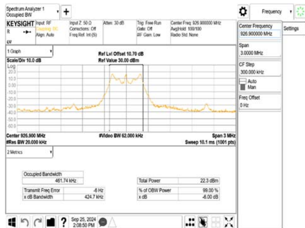
IC OBW_FSK_100Kbps_HighCH-926.9MHz
