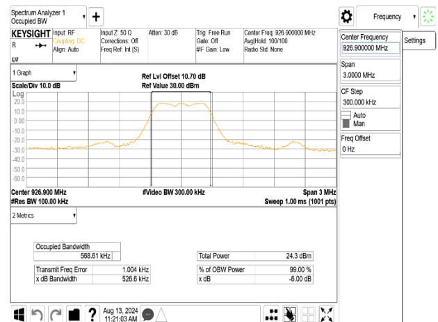
OBW_FSK_100Kbps_HighCH-926.9MHz
