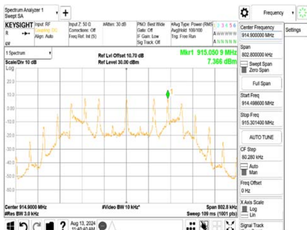
PSD_FSK_100Kbps_MidCH-914.9MHz
