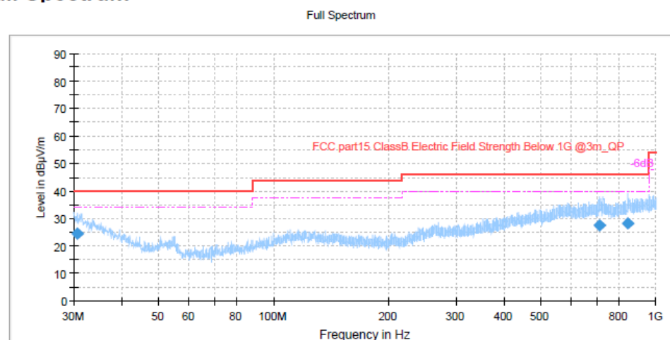
Figure 14: Spectral Diagrams, Radiated Emission, 30MHz-1000MHz, Vertical, for Battery Charging mode
