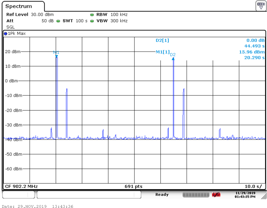
Figure 8: Dwell time
