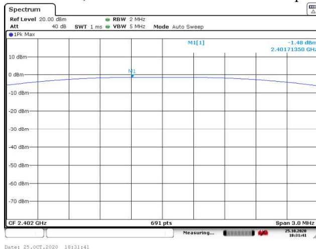
Figure 3: Maximum peak Conducted Output Power
