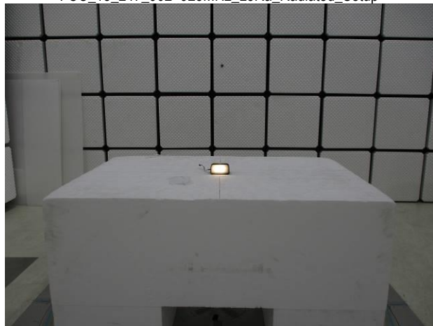
FCC_15_247_902~928MHz_LoRa_Radiated_Setup
