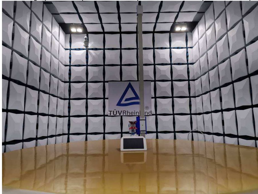
Photograph 1: Set-up for Radiated Spurious Emissions (1GHz-18GHz)
