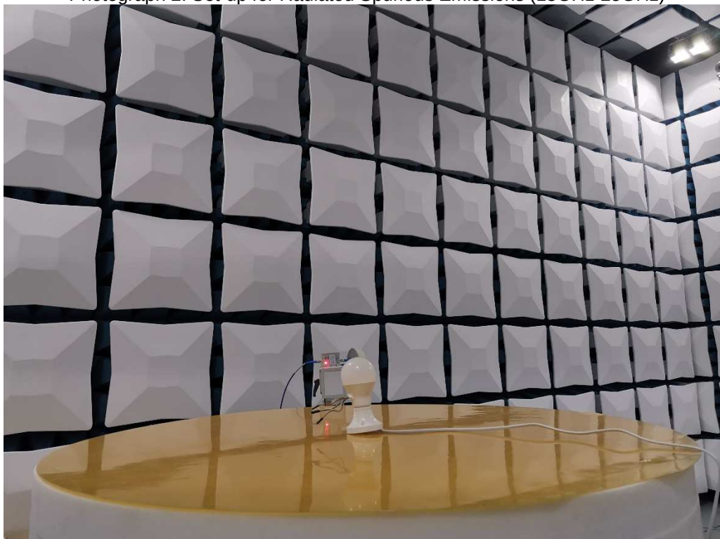
Photograph 2: Set-up for Radiated Spurious Emissions (18GHz-25GHz)
