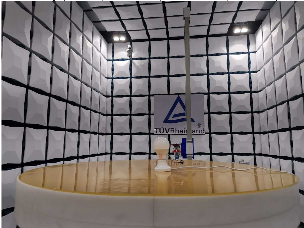
Photograph 1: Set-up for Radiated Spurious Emissions (1GHz-18GHz)
