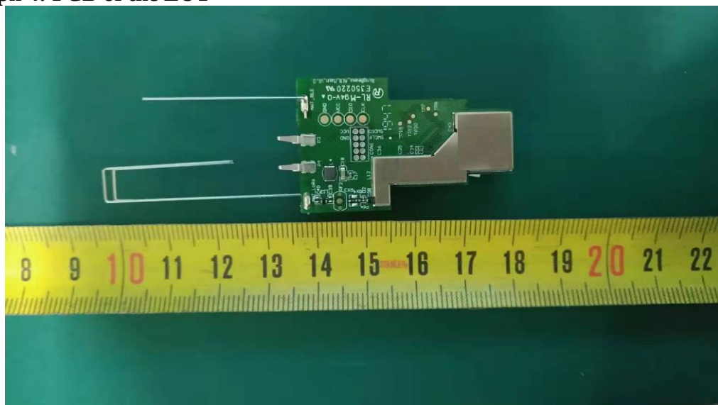
Photograph 4: PCB of the EUT
