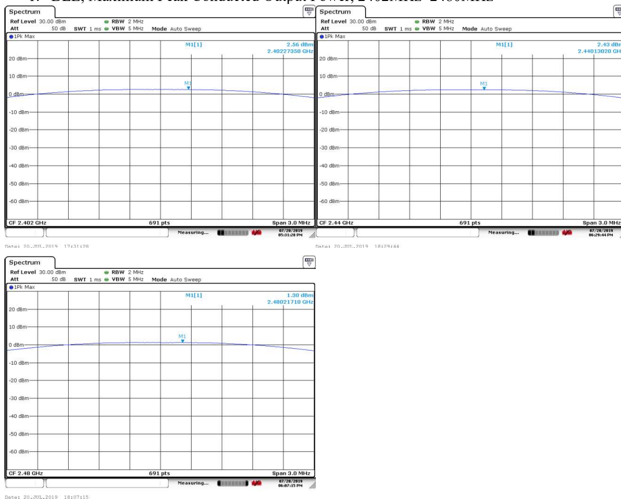
Figure 3: Maximum peak Conducted Output Power
