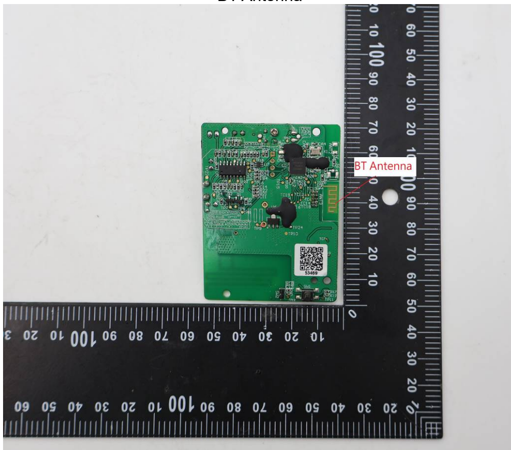
BT Antenna
