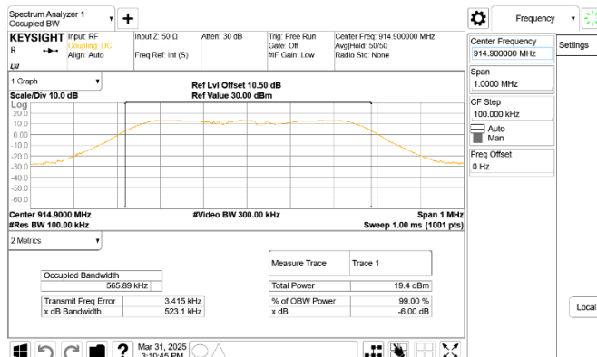
OBW_FSK 100Kbps_MidCH-914.9MHz
