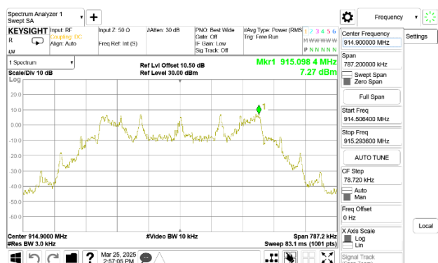
PSD_FSK 100Kbps_MidCH-914.9MHz
