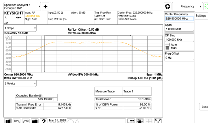
OBW_FSK 100Kbps_HighCH-926.9MHz
