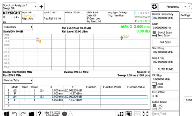
FSK 100Kbps_LowCH-902.9MHz
