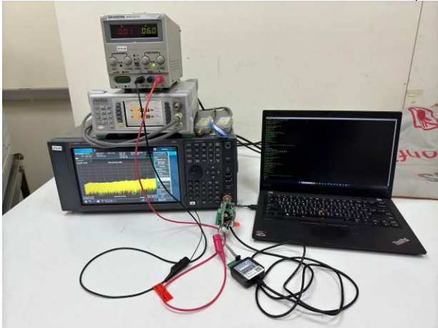
FCC_15_247+RSS 247_902~928MHz_LoRa_Radiated_Setup
