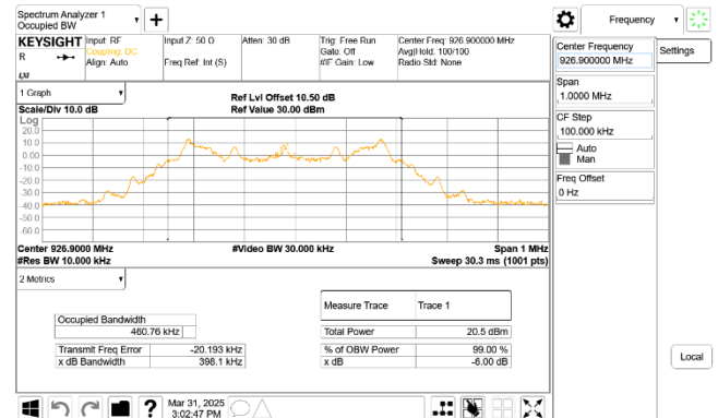
IC OBW_FSK 100Kbps _HighCH-926.9MHz
