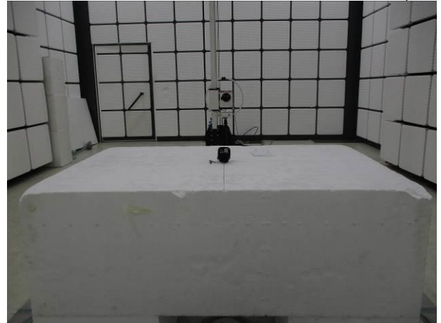
FCC_15_247+RSS 247_902~928MHz_LoRa_Radiated_Setup
