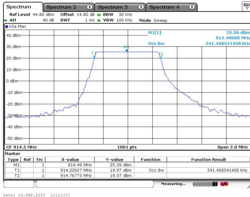
99% Occupied Bandwidth Plot on Channel 914.5
