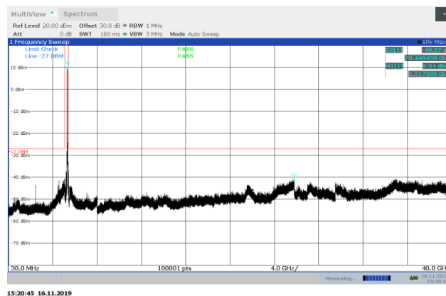
Figure 8.7-26: Conducted spurious emissions 30 MHz – 40 GHz high channel, 802.11a
