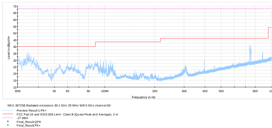
Figure 8.7-6: Radiated spurious emissions 30 MHz – 1 GHz mid channel, 802.11a
