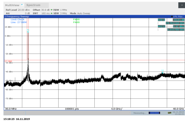
Figure 8.7-28: Conducted spurious emissions 30 MHz – 40 GHz high channel, 802.11n
