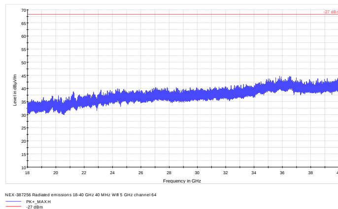
Figure 8.7-19: Radiated spurious emissions 18 - 40 GHz high channel, 802.11n
