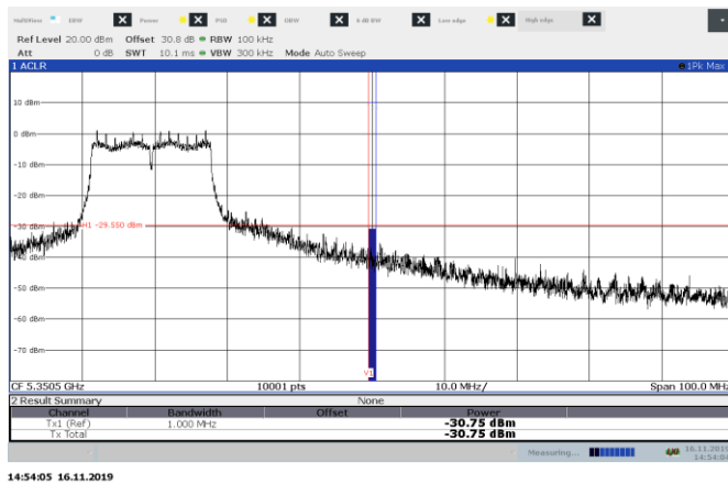
Figure 8.7-20: Conducted emissions at band edge measurement, channel 64, 802.11a
