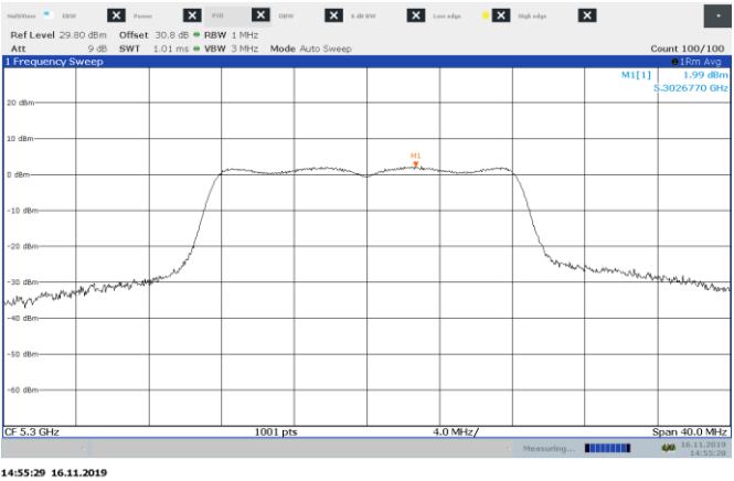
Figure 8.6-2: Sample plot for PSD on 802.11a
