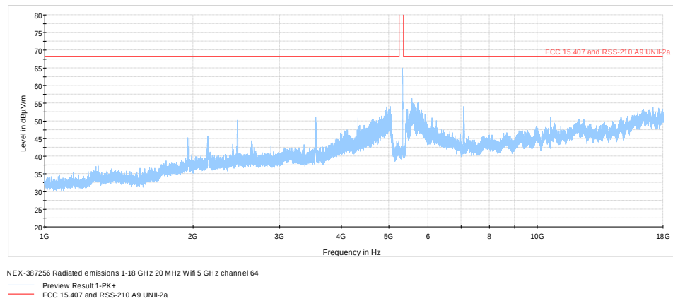
Figure 8.7-12: Radiated spurious emissions 1 - 18 GHz high channel, 802.11a
