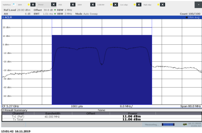
Figure 8.6-3: Sample plot for power on 802.11n
