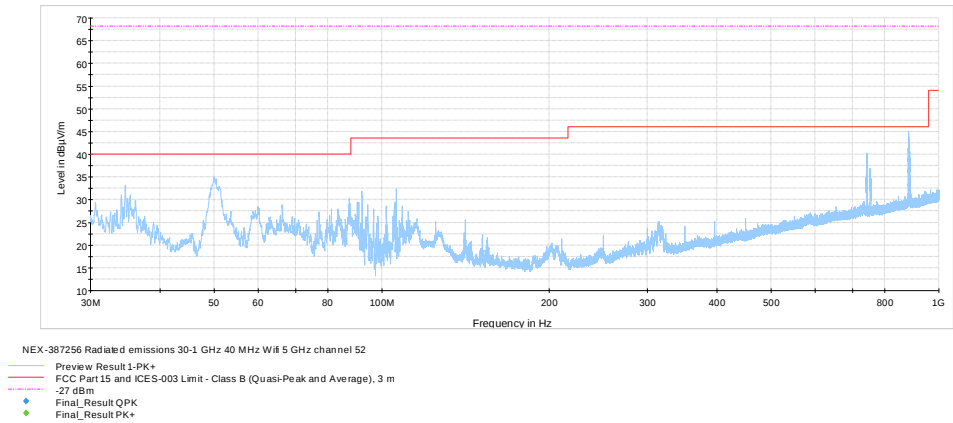
Figure 8.7-8: Radiated spurious emissions 30 MHz – 1 GHz low channel, 802.11n
