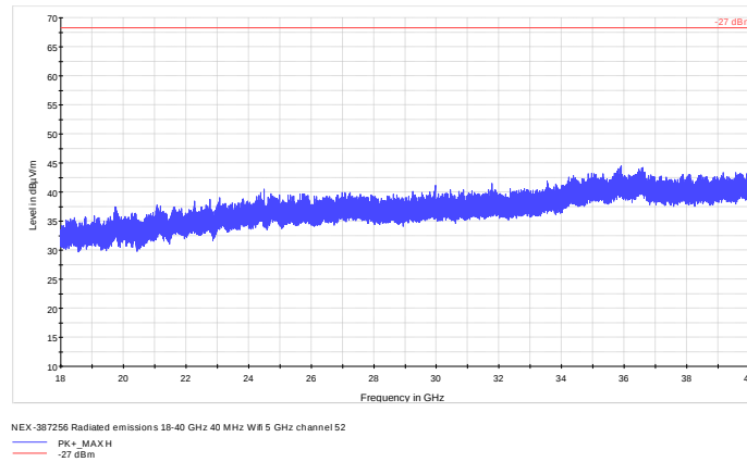
Figure 8.7-18: Radiated spurious emissions 18 - 40 GHz low channel, 802.11n
