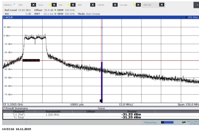
Figure 8.7-22: Conducted emissions at band edge measurement, channel 60, 802.11a
