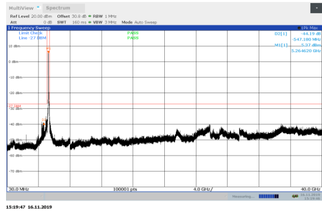
Figure 8.7-27: Conducted spurious emissions 30 MHz – 40 GHz low channel, 802.11n
