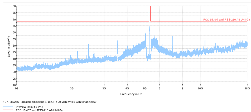
Figure 8.7-11: Radiated spurious emissions 1 - 18 GHz mid channel, 802.11a
