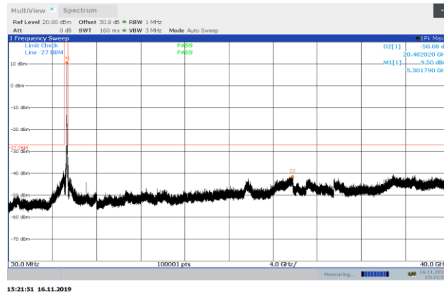
Figure 8.7-25: Conducted spurious emissions 30 MHz – 40 GHz mid channel, 802.11a
