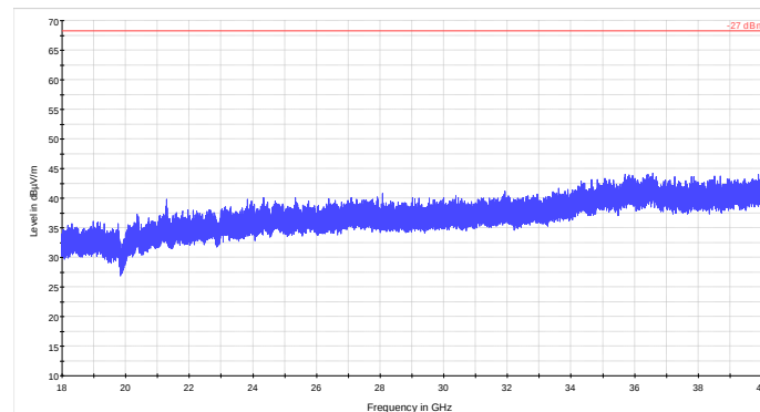
Figure 8.7-16: Radiated spurious emissions 18 - 40 GHz mid channel, 802.11a
