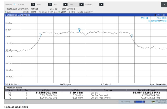
Figure 8.5-3: 99 % bandwidth on 802.11a, sample plot
