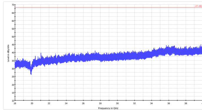
Figure 8.7-15: Radiated spurious emissions 18 - 40 GHz low channel, 802.11a
