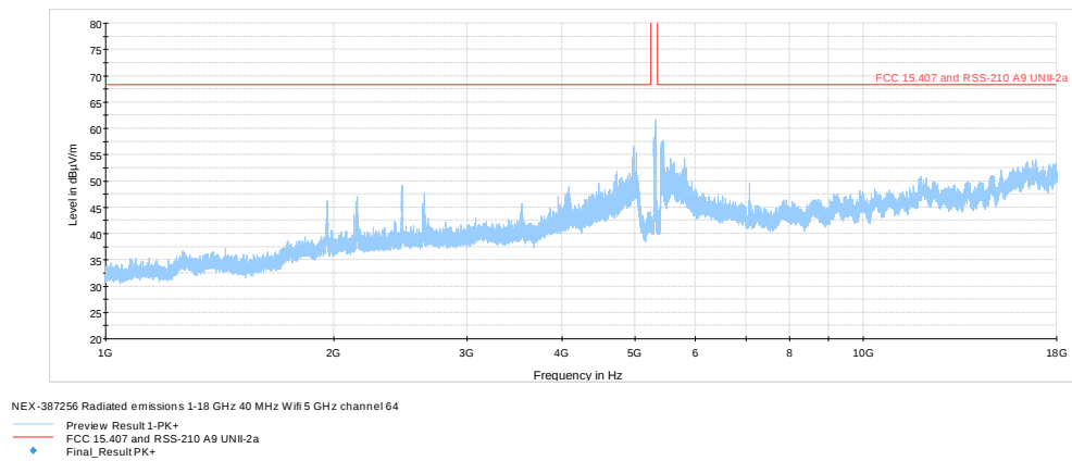
Figure 8.7-14: Radiated spurious emissions 1 - 18 GHz high channel, 802.11n
