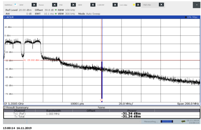
Figure 8.7-23: Conducted emissions at band edge measurement, channel 52, 802.11n
