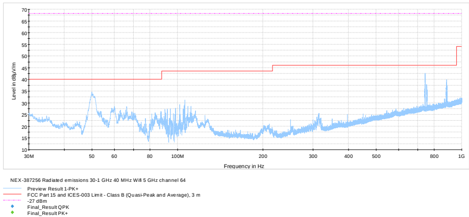
Figure 8.7-9: Radiated spurious emissions 30 MHz – 1 GHz high channel, 802.11n
