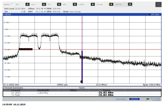
Figure 8.7-21: Conducted emissions at band edge measurement, channel 64, 802.11n
