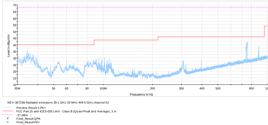
Figure 8.7-5: Radiated spurious emissions 30 MHz – 1 GHz low channel, 802.11a
