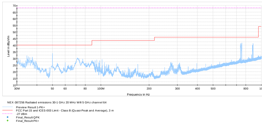
Figure 8.7-7: Radiated spurious emissions 30 MHz – 1 GHz high channel, 802.11a
