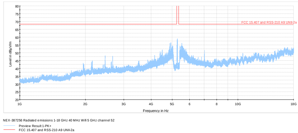
Figure 8.7-13: Radiated spurious emissions 1 - 18 GHz low channel, 802.11n
