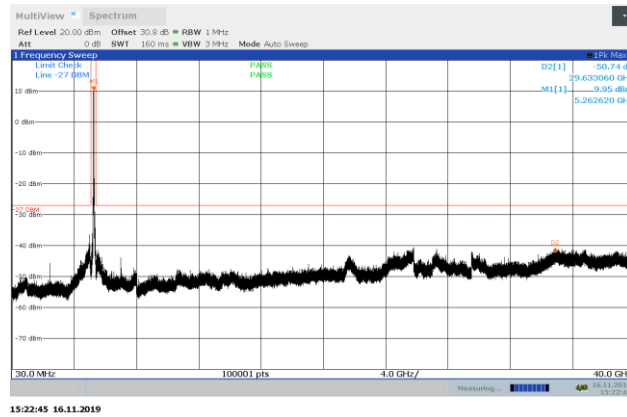
Figure 8.7-24: Conducted spurious emissions 30 MHz – 40 GHz low channel, 802.11a
