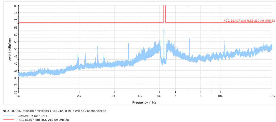
Figure 8.7-10: Radiated spurious emissions 1 - 18 GHz low channel, 802.11a
