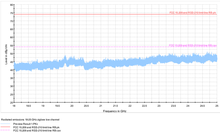
Figure 8.7-11: Radiated spurious emissions 18 – 25 GHz, low channel
