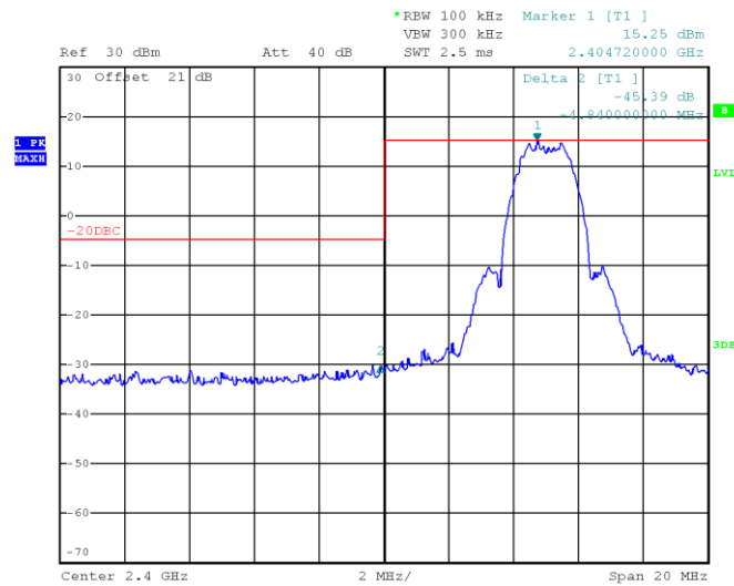
Figure 8.7-17: Conducted spurious emissions at the lower band edge
