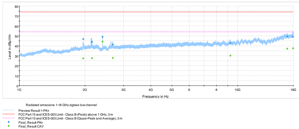
Figure 8.7-8: Radiated spurious emissions 1 – 18 GHz, low channel
