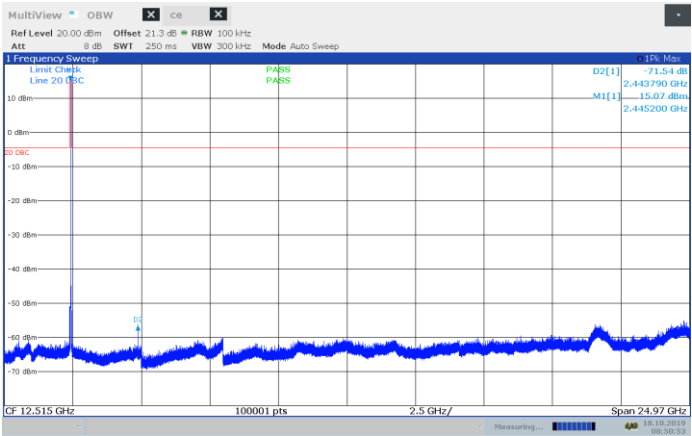
Figure 8.7-15: Conducted spurious emissions on mid channel
