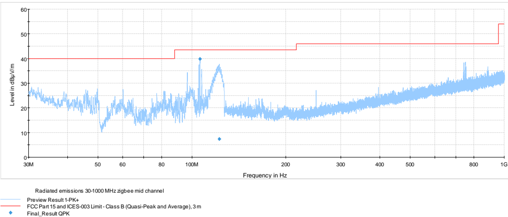
Figure 8.7-6: Radiated spurious emissions 30 MHz – 1 GHz, mid channel
