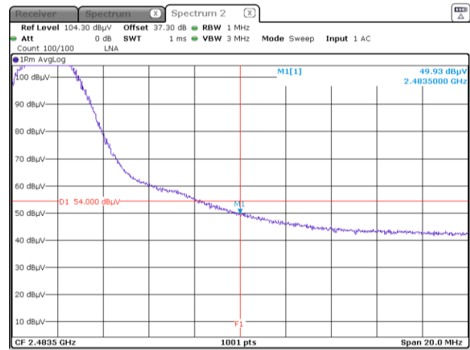
Figure 8.7-2: Radiated spurious emissions at the upper band edge, average
