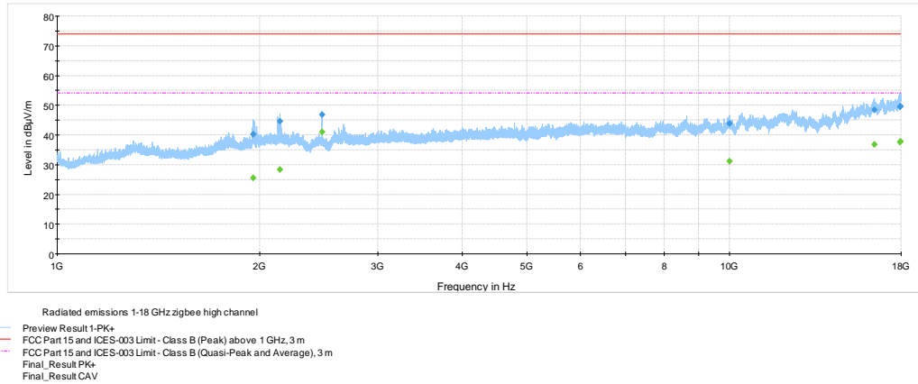
Figure 8.7-10: Radiated spurious emissions 1 – 18 GHz, high channel
