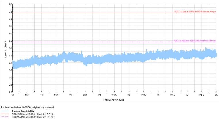
Figure 8.7-13: Radiated spurious emissions 18 – 25 GHz, high channel
