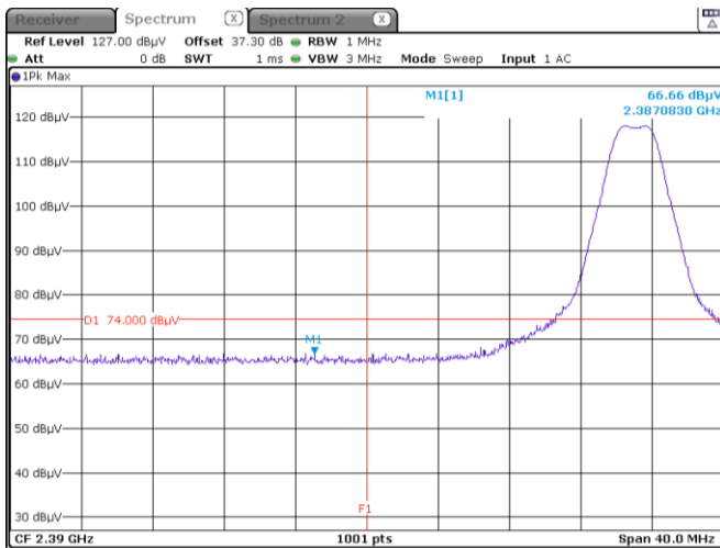
Figure 8.7-3: Radiated restricted bands spurious emissions at 2.39 GHz, peak
