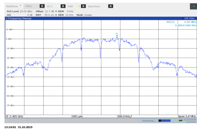
Figure 8.8-1: PSD plot on low channel
