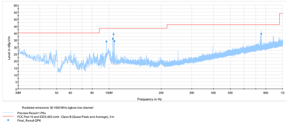
Figure 8.7-5: Radiated spurious emissions 30 MHz – 1 GHz, low channel
