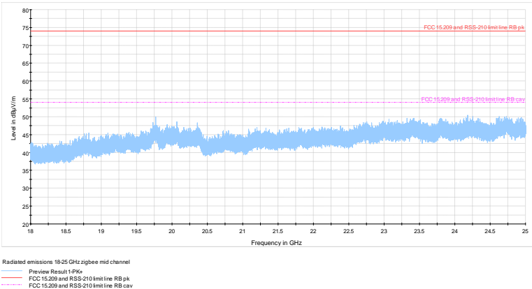
Figure 8.7-12: Radiated spurious emissions 18 – 25 GHz, mid channel
