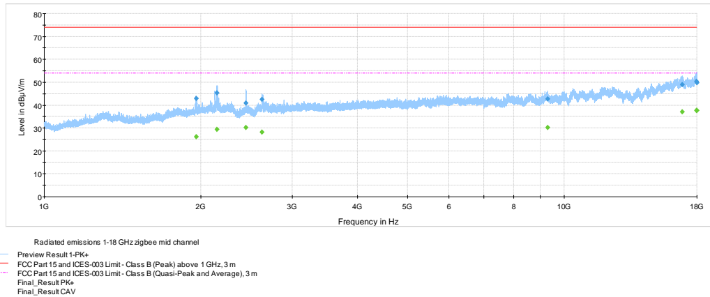
Figure 8.7-9: Radiated spurious emissions 1 – 18 GHz, mid channel
