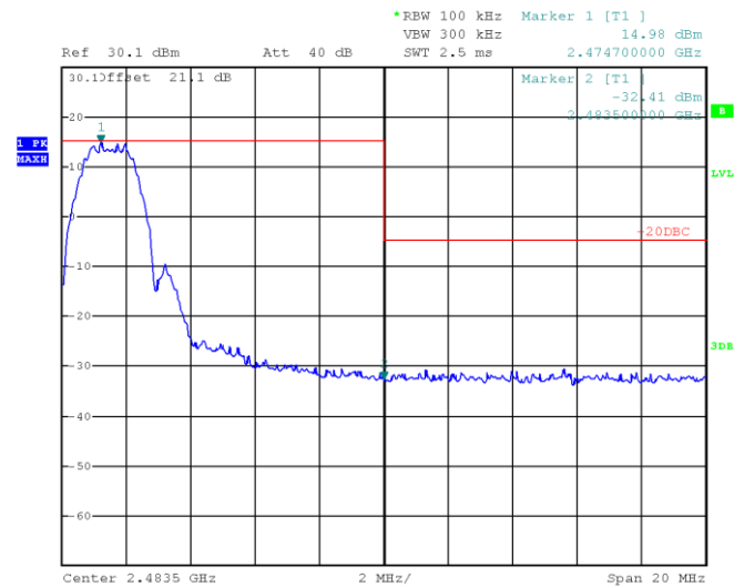
Figure 8.7-18: Conducted spurious emissions at the upper band edge
