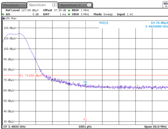
Figure 8.7-1: Radiated spurious emissions at the upper band edge, peak
