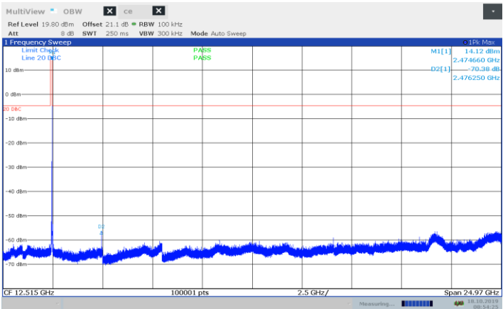
Figure 8.7-16: Conducted spurious emissions on high channel
