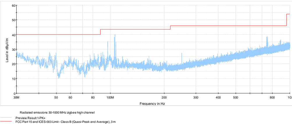
Figure 8.7-7: Radiated spurious emissions 30 MHz – 1 GHz, high channel
