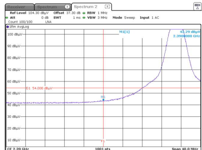
Figure 8.7-4: Radiated restricted bands spurious emissions at 2.39 GHz, average
