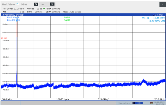
Figure 8.7-14: Conducted spurious emissions on low channel
