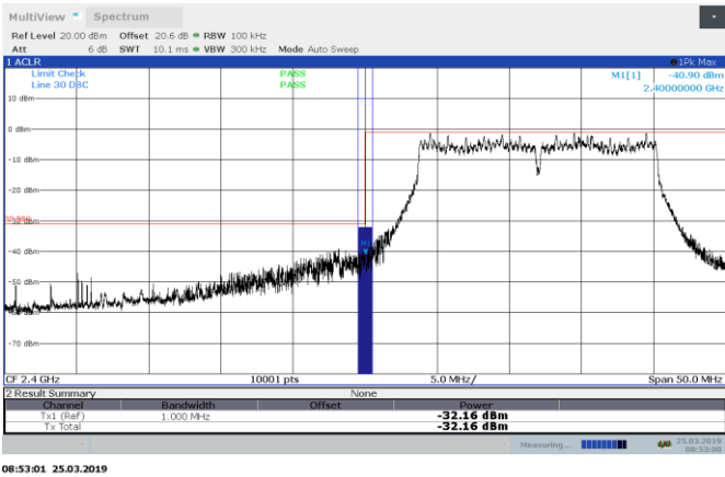
Figure 8.7-55: Conducted band edge emissions for 802.11g, low channel
