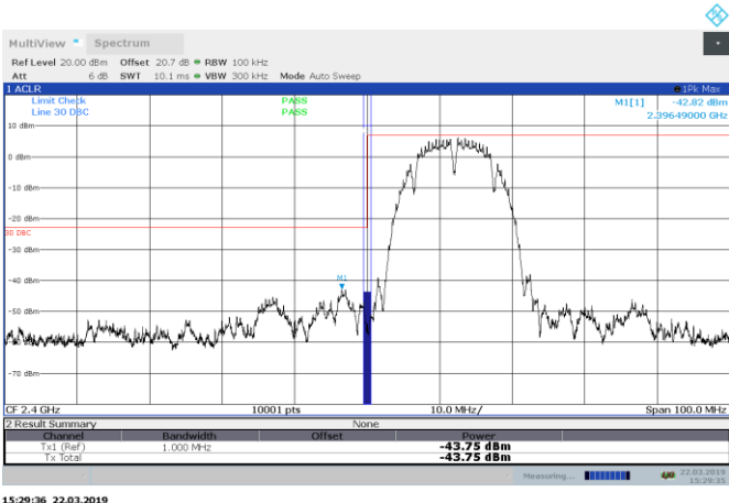
Figure 8.7-53: Conducted band edge emissions for 802.11b, low channel
