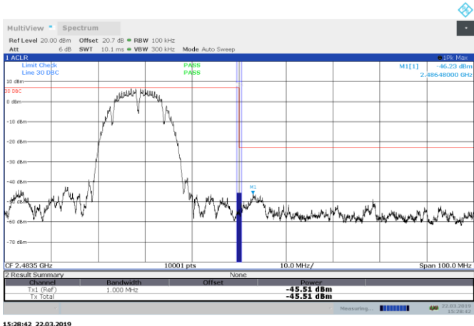
Figure 8.7-54: Conducted band edge emissions for 802.11b, high channel
