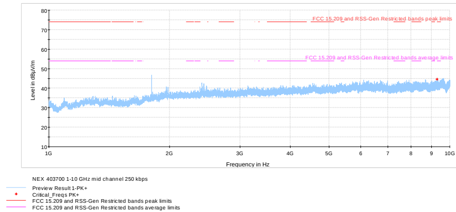
Figure 8.8-41: Radiated spurious emissions 1 – 10 GHz on mid channel, FSK 250kbps
