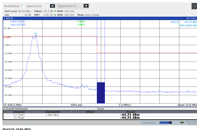
Figure 8.8-44: Conducted Band-edge on 920 MHz channel, Z-Wave Long Range
