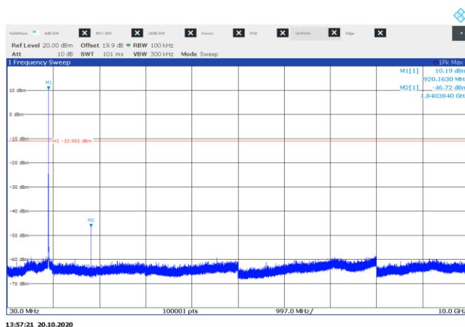
Figure 8.8-46: Conducted spurious emissions on 920 MHz channel, Z-Wave Long Range
