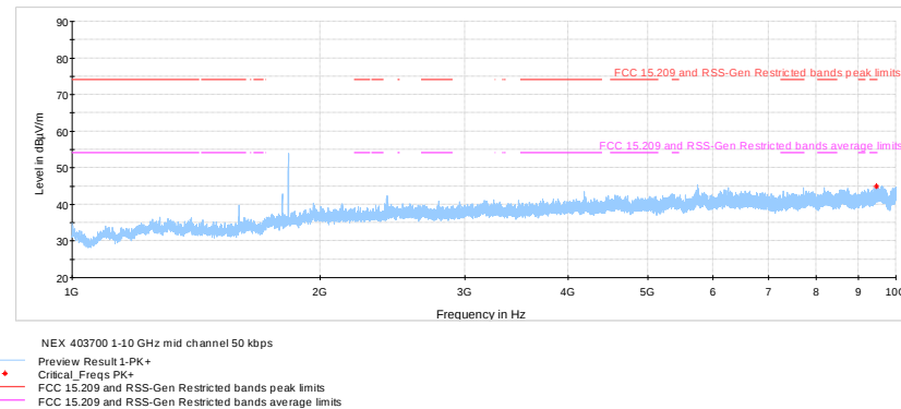
Figure 8.8-13: Radiated spurious emissions 1 – 10 GHz on mid channel, FSK 50kbps
