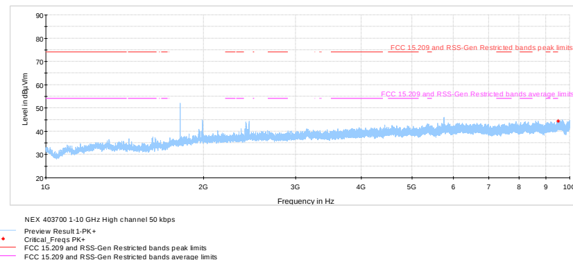
Figure 8.8-14: Radiated spurious emissions 1 – 10 GHz on high channel, FSK 50kbps
