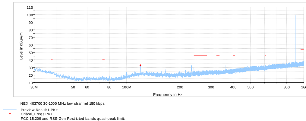
Figure 8.8-23: Radiated spurious emissions 30 MHz – 1 GHz on low channel, FSK 150kbps
