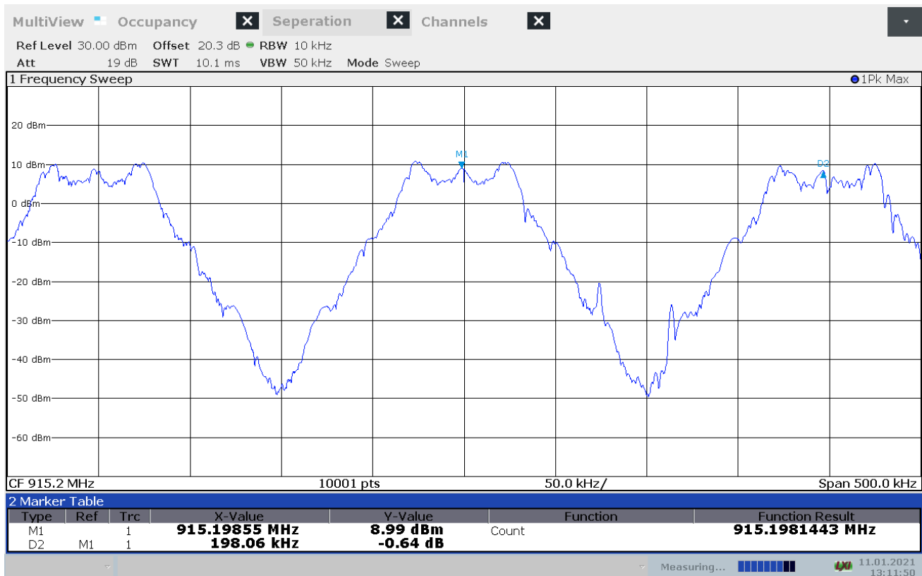
Figure 8.4-7: Carrier frequency separation
