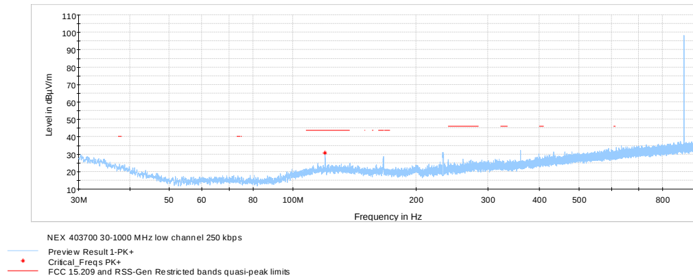
Figure 8.8-37: Radiated spurious emissions 30 MHz – 1 GHz on low channel, FSK 250kbps
