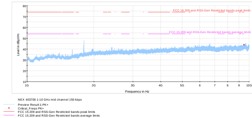
Figure 8.8-27: Radiated spurious emissions 1 – 10 GHz on mid channel, FSK 150kbps
