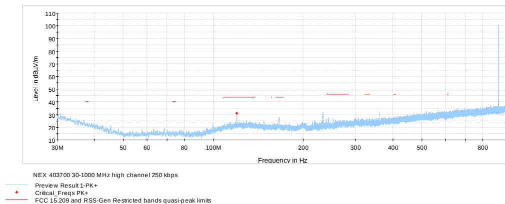
Figure 8.8-39: Radiated spurious emissions 30 MHz – 1 GHz on high channel, FSK 250kbps
