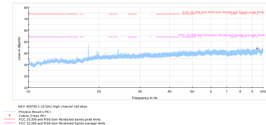
Figure 8.8-28: Radiated spurious emissions 1 – 10 GHz on high channel, FSK 150kbps
