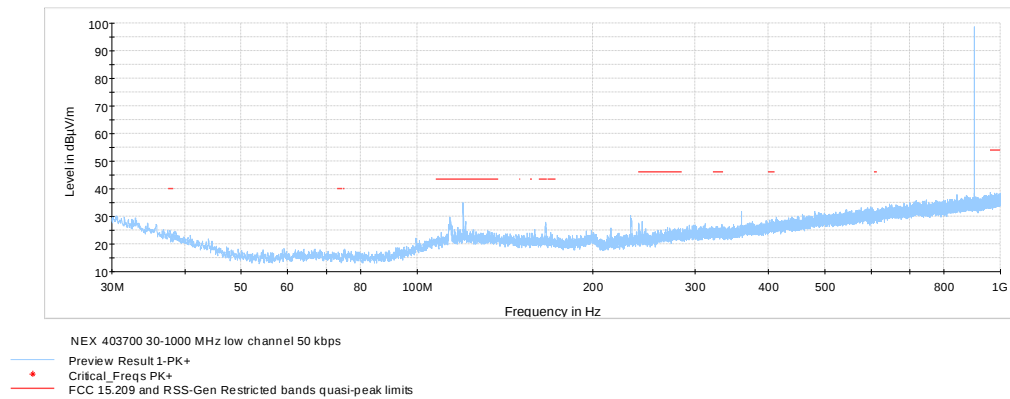
Figure 8.8-9: Radiated spurious emissions 30 MHz – 1 GHz on low channel, FSK 50kbps
