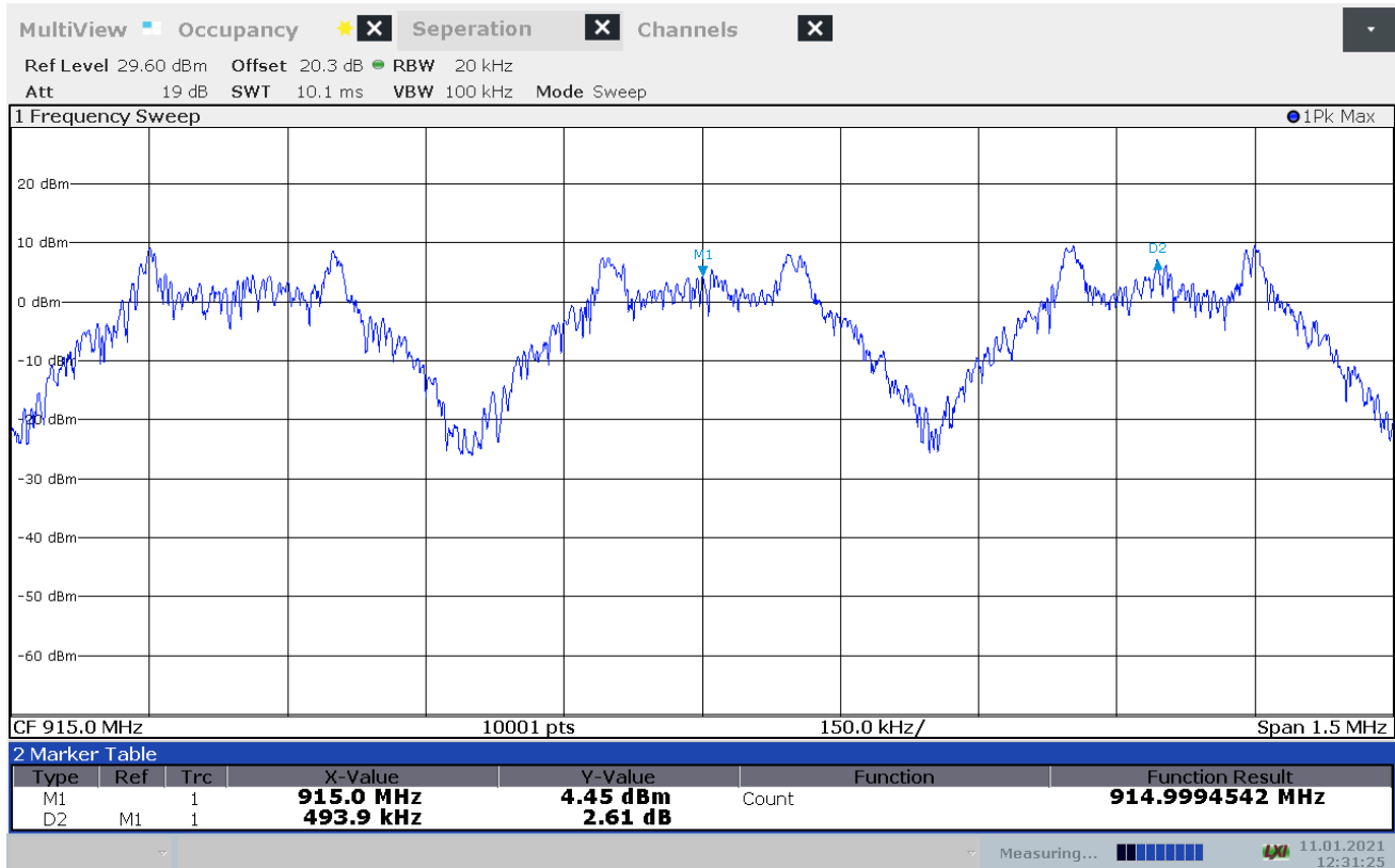
Figure 8.4-27: Carrier frequency separation
