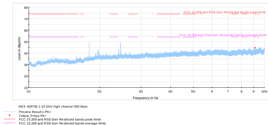
Figure 8.8-42: Radiated spurious emissions 1 – 10 GHz on high channel, FSK 250kbps
