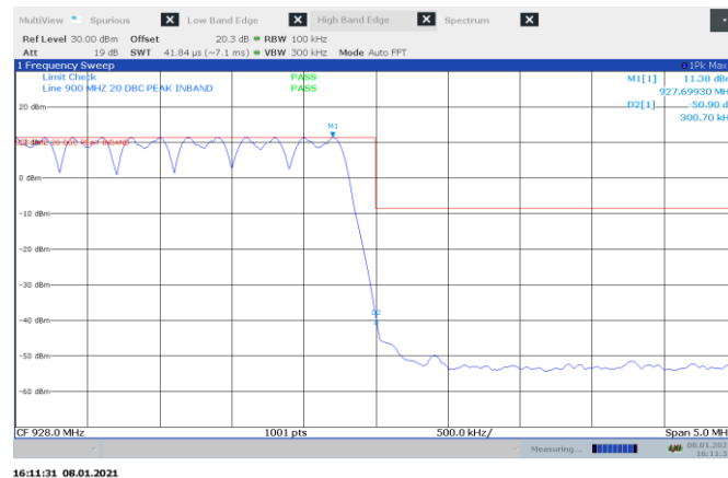
Figure 8.8-18: Conducted High Band-edge on Hopping, FSK 150kbps
