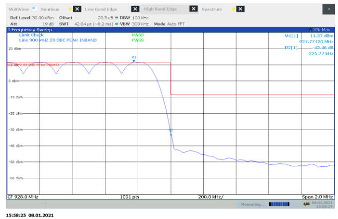
Figure 8.8-4: Conducted High Band-edge on hopping, FSK 50kbps
