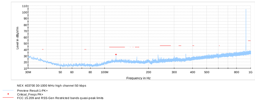
Figure 8.8-11: Radiated spurious emissions 30 MHz – 1 GHz on high channel, FSK 50kbps
