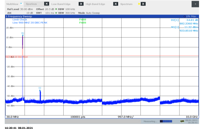
Figure 8.8-36: Conducted spurious emissions on hopping, FSK 250kbps
