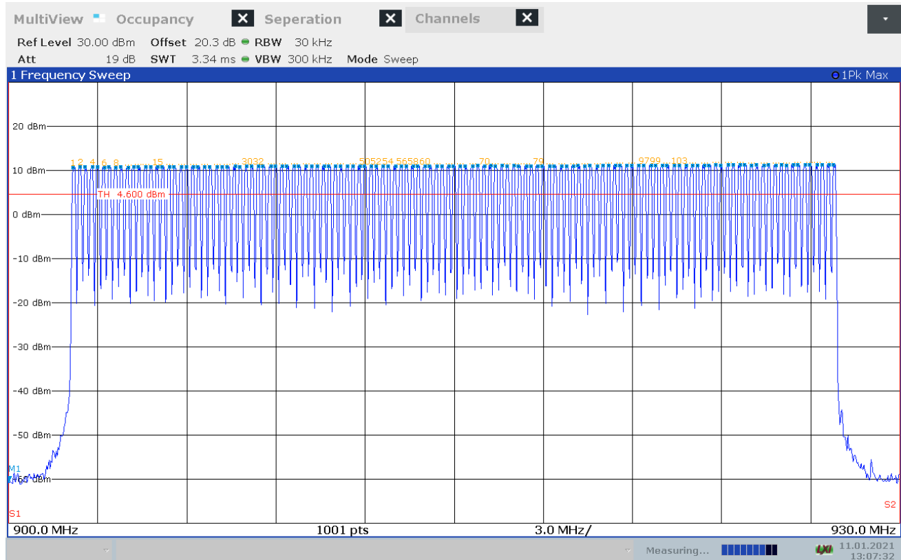
Figure 8.4-9: Number of hopping frequencies = 128
