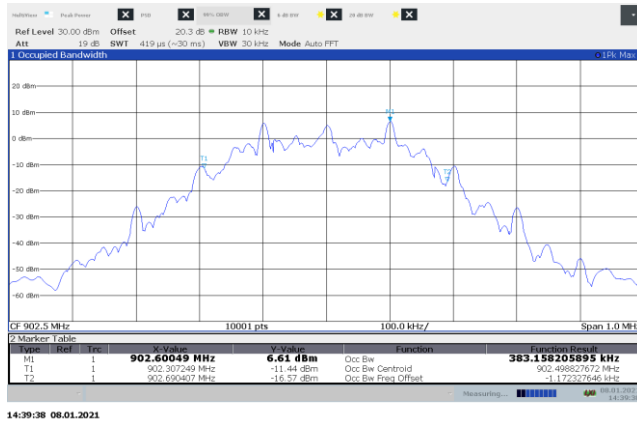
Figure 8.4-24: 99% OBW on low channel, 250 kbps
