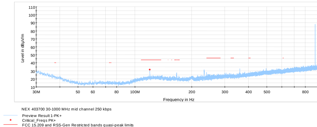
Figure 8.8-38: Radiated spurious emissions 30 MHz – 1 GHz on mid channel, FSK 250kbps
