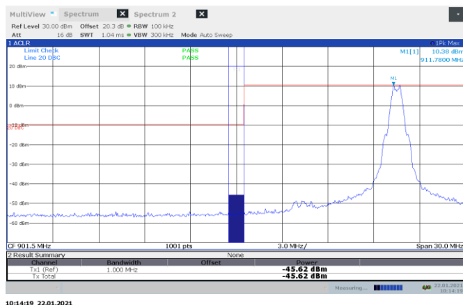
Figure 8.8-43: Conducted Band-edge on 912 MHz channel, Z-Wave Long Range
