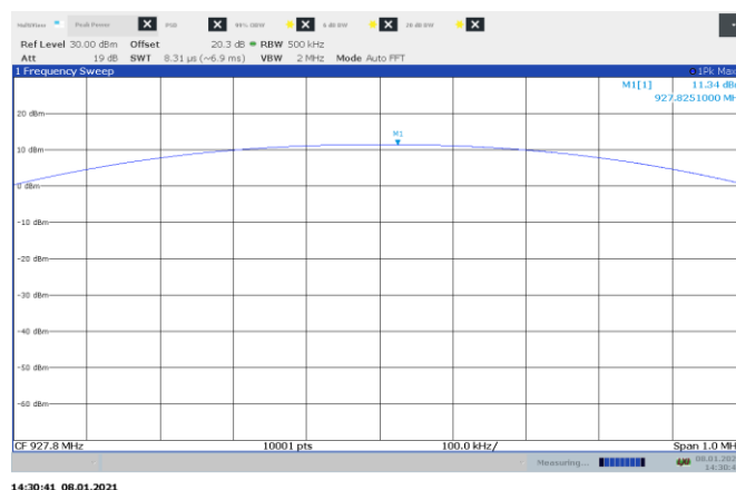
Figure 8.5-3: Output power on high channel, 50 kbps
