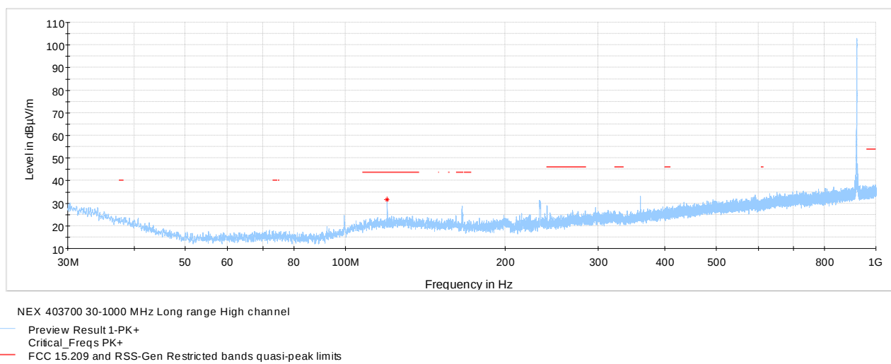
Figure 8.8-48: Radiated spurious emissions 30 MHz – 1 GHz, on 920 MHz channel, Z-Wave Long Range
