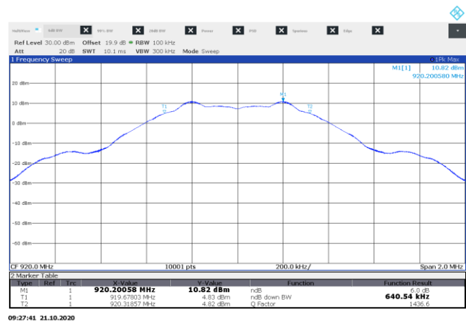
Figure 8.6-2: 6 dB bandwidth on 920 MHz channel, Z-Wave Long Range
