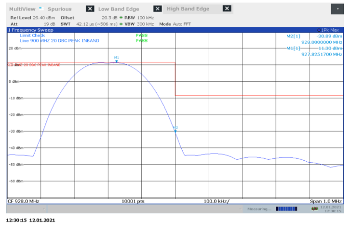
Figure 8.8-2: Conducted Band-edge on high channel, FSK 50kbps
