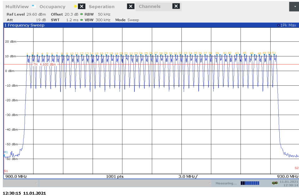
Figure 8.4-28: Number of hopping frequencies = 51
