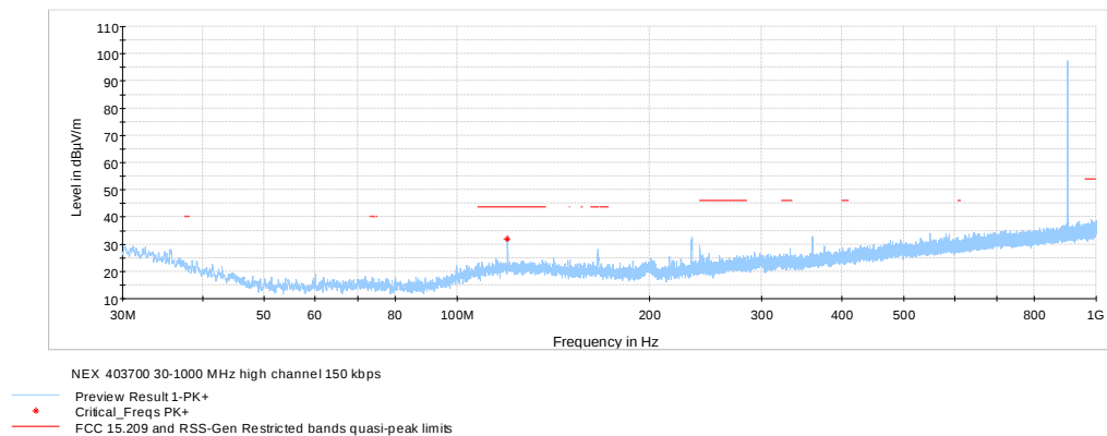
Figure 8.8-25: Radiated spurious emissions 30 MHz – 1 GHz on high channel, FSK 150kbps
