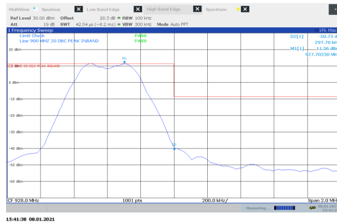
Figure 8.8-16: Conducted Band-edge on high channel, FSK 150kbps
