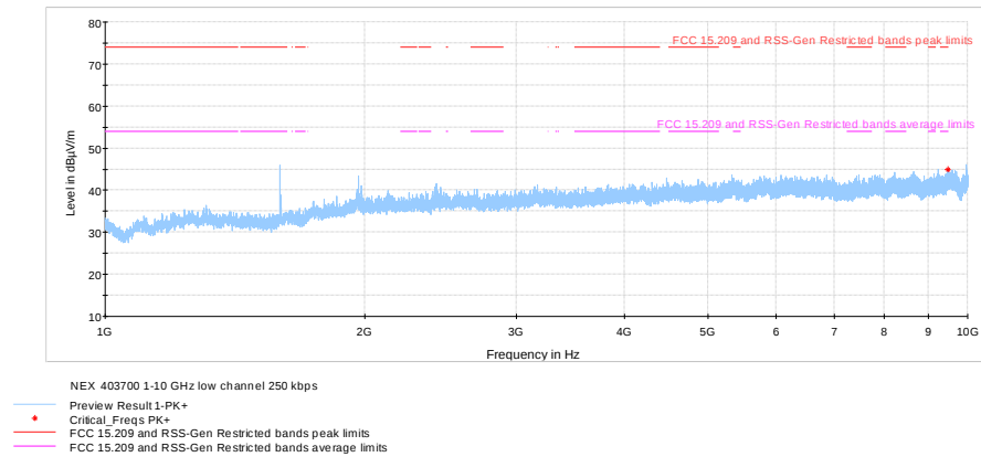
Figure 8.8-40: Radiated spurious emissions 1 – 10 GHz on low channel, FSK 250kbps
