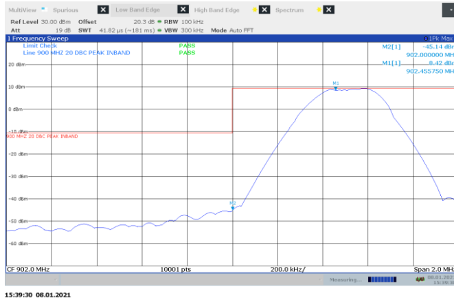
Figure 8.8-29: Conducted Band-edge on low channel, FSK 250kbps
