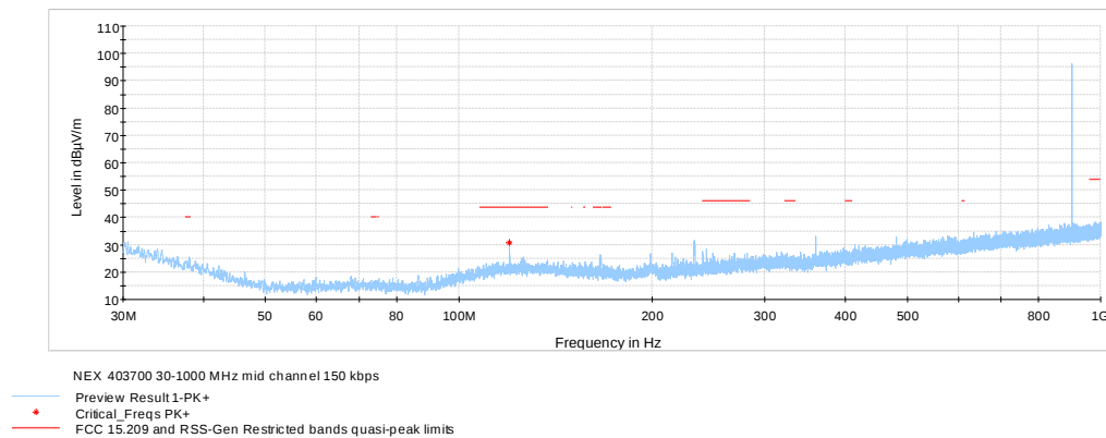
Figure 8.8-24: Radiated spurious emissions 30 MHz – 1 GHz on mid channel, FSK 150kbps
