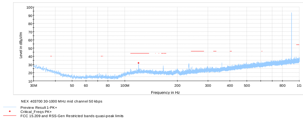
Figure 8.8-10: Radiated spurious emissions 30 MHz – 1 GHz on mid channel, FSK 50kbps
