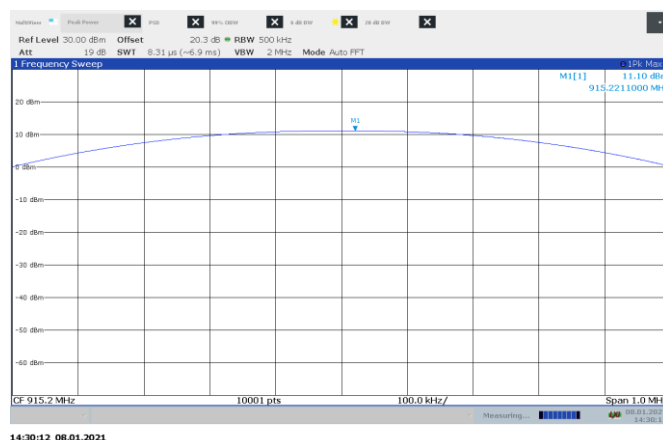
Figure 8.5-2: Output power on mid channel, 50 kbps
