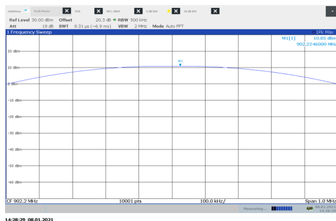
Figure 8.5-1: Output power on low channel, 50 kbps
