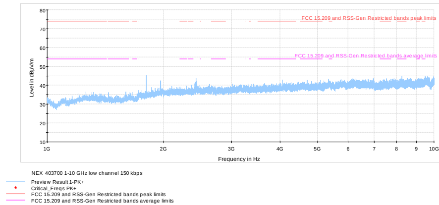
Figure 8.8-26: Radiated spurious emissions 1 – 10 GHz on low channel, FSK 150kbps
