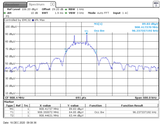
Figure 8.6-2: 99 % occupied bandwidth, 908.4 MHz
