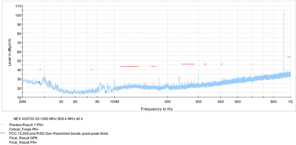
Figure 8.5-3: Spurious emissions below 1 GHz, 908.42 MHz
