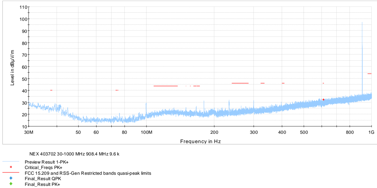
Figure 8.5-1: Spurious emissions below 1 GHz, 908.4 MHz
