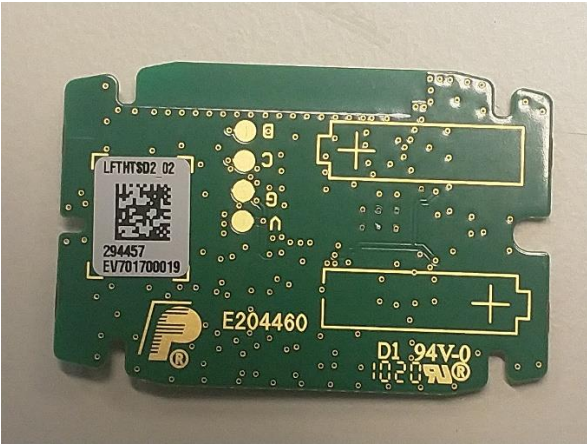
1 PWB bottom
