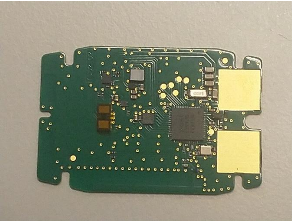
2 PWB top
