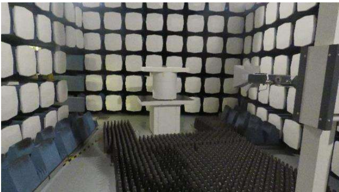
Picture 4 Radiated test setup, Common view, 1-18GHz
