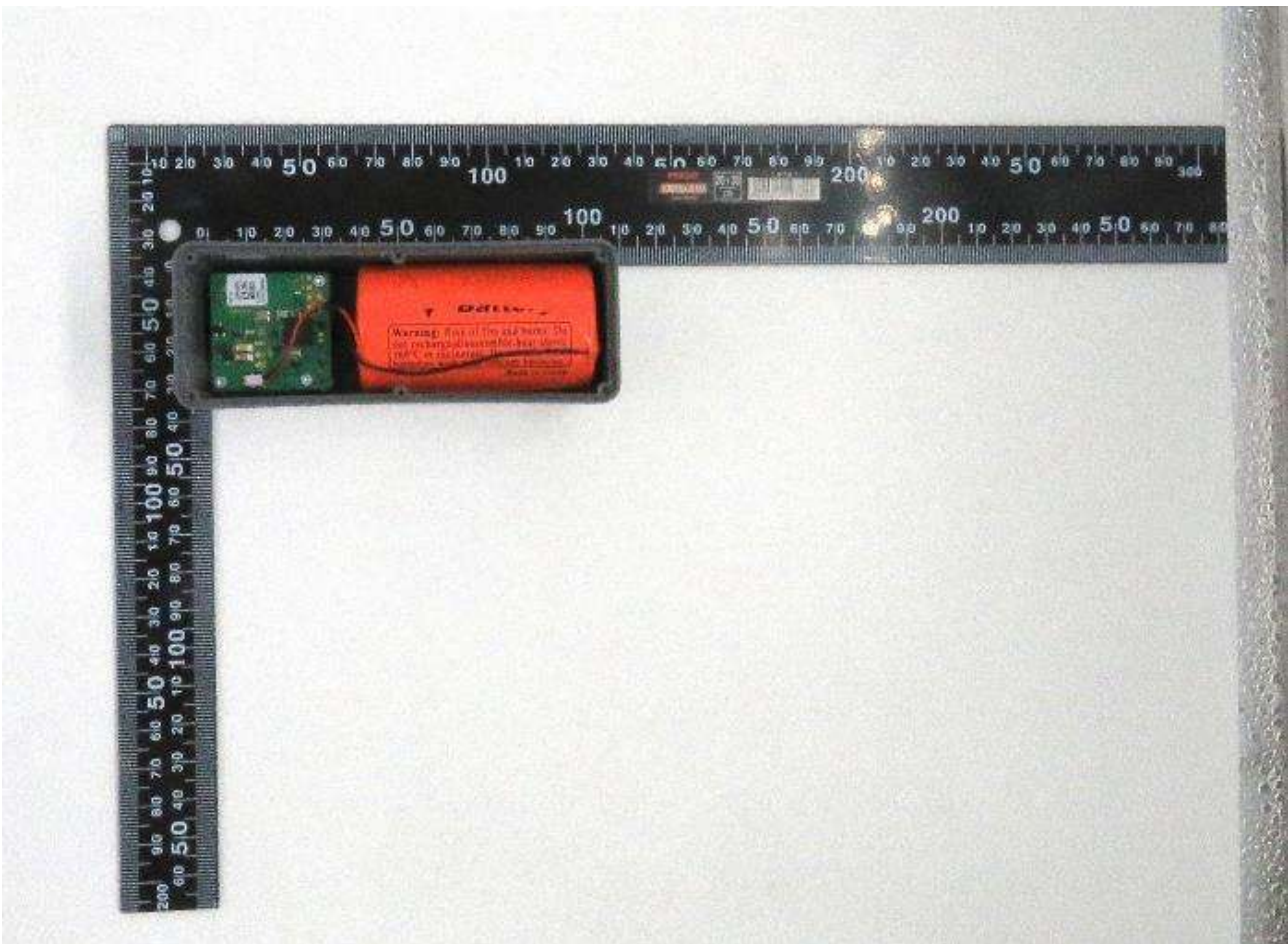
Picture 18 EUT PCB and battery inside B cover
