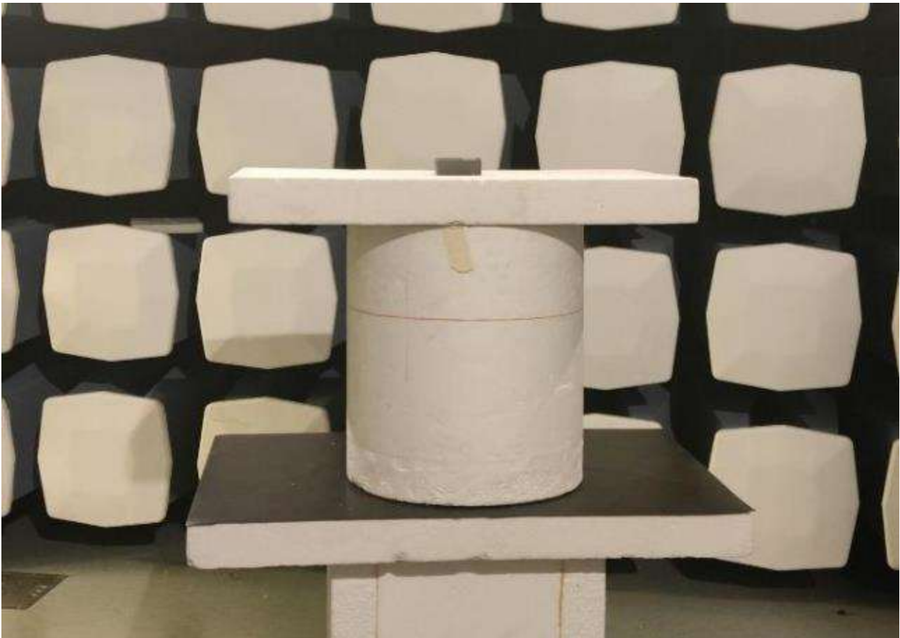
Picture 8 Radiated test setup, Front view, 18 - 26GHz
