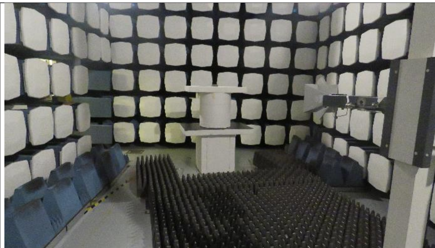
Picture 8, Radiated Spurious Emissions, common setup, TX, 1 – 26 GHz
