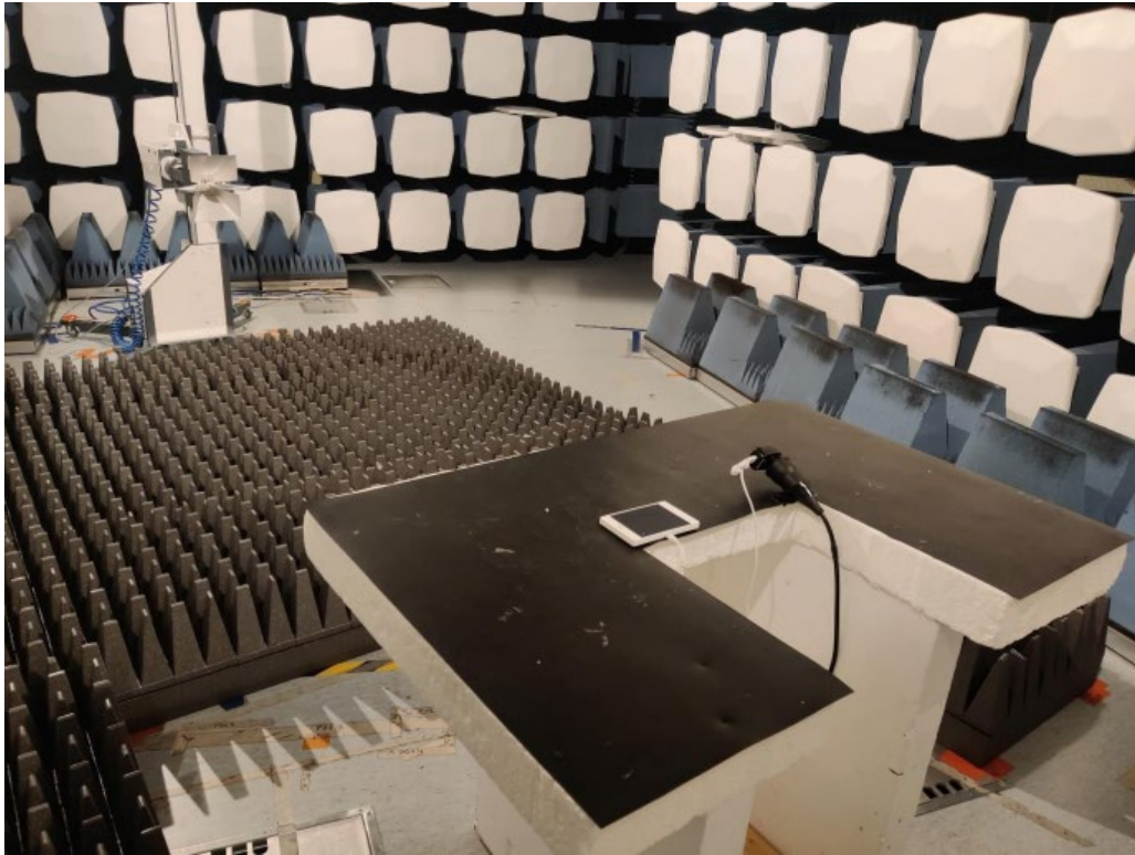
Radiated emission common setup, 1-12,75 GHz
