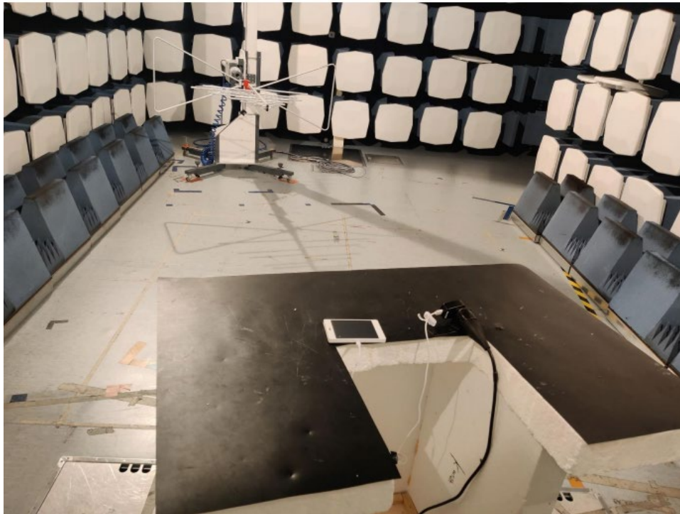
Radiated emission common setup, 30-1000MHz
