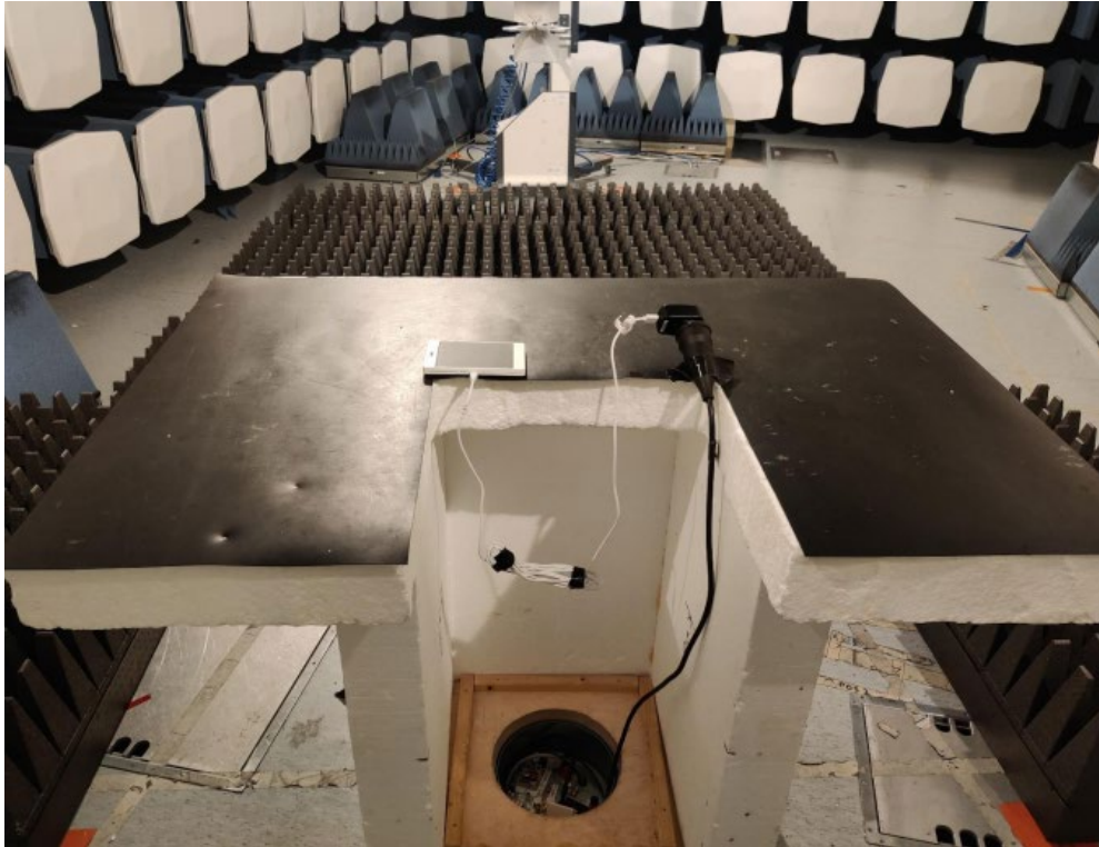
Radiated emission EUT setup back view, 1-12,75 GHz
