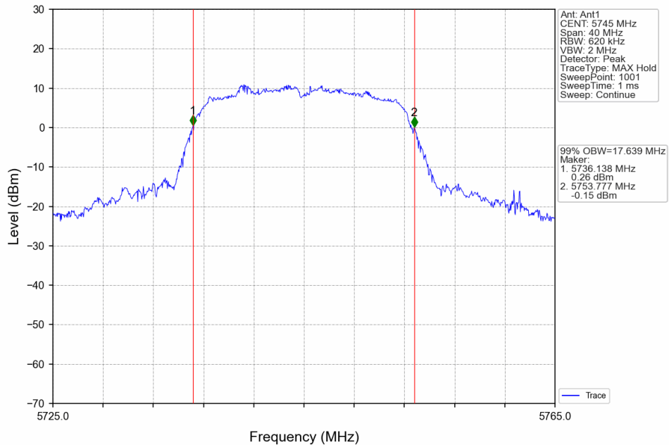
802.11a_LCH_5745MHz_Ant1_NTNV
