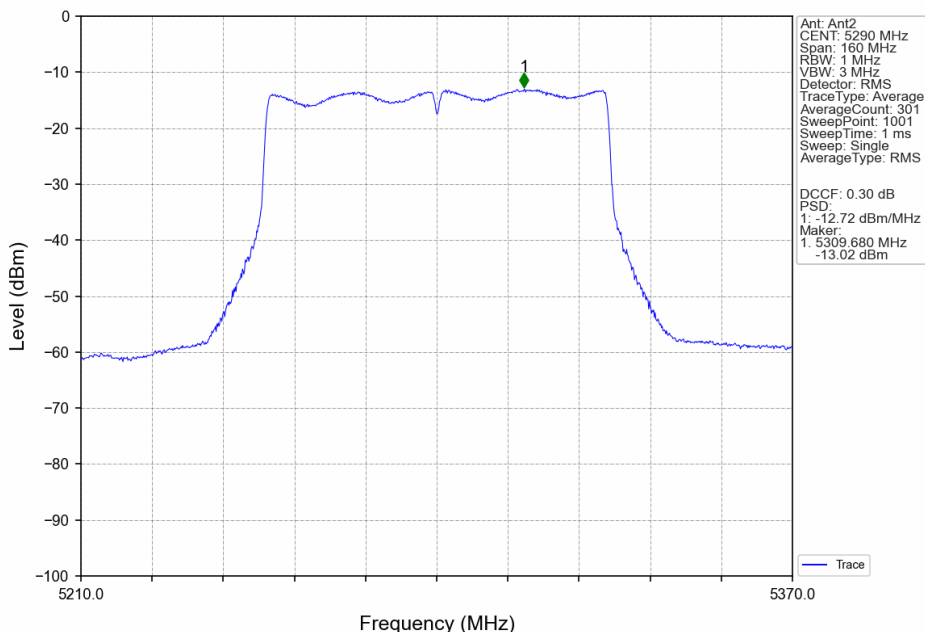
802.11ac(VHT80)_MCH_5290MHz_MIMO_NTNV
