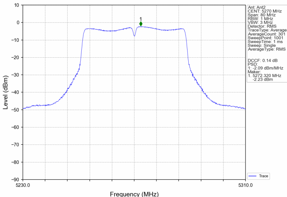
802.11ac(VHT40)_LCH_5270MHz_MIMO_NTNV
