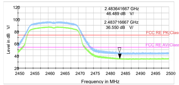
802.11g-Channel 11 Peak &amp; Average
