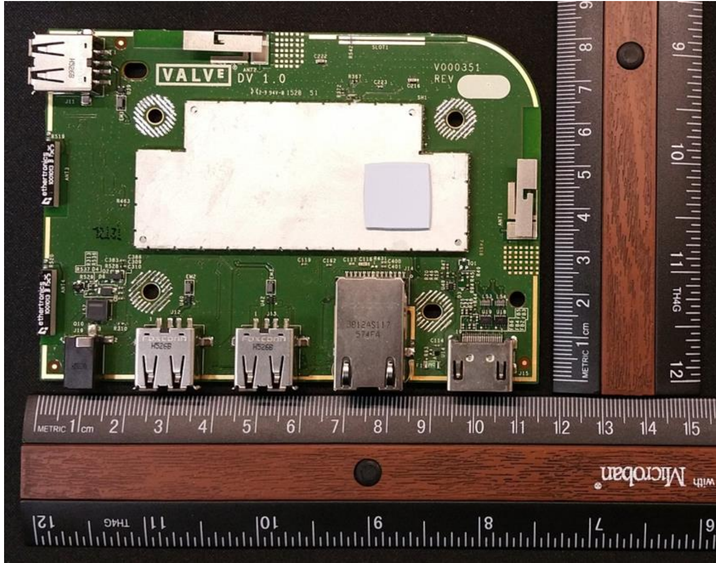
Motherboard Top
