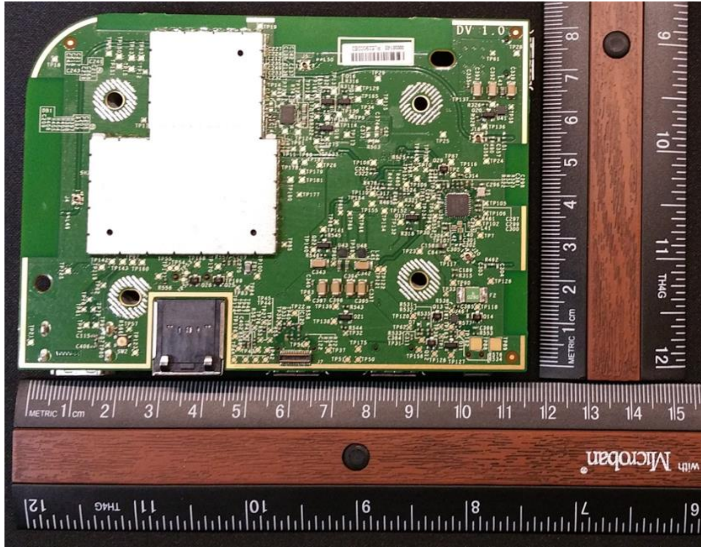
Motherboard Bottom
