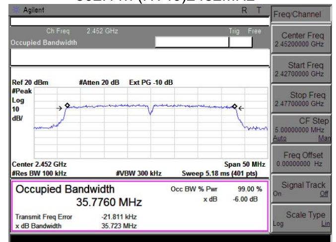
802.11n (HT40)2452MHz
