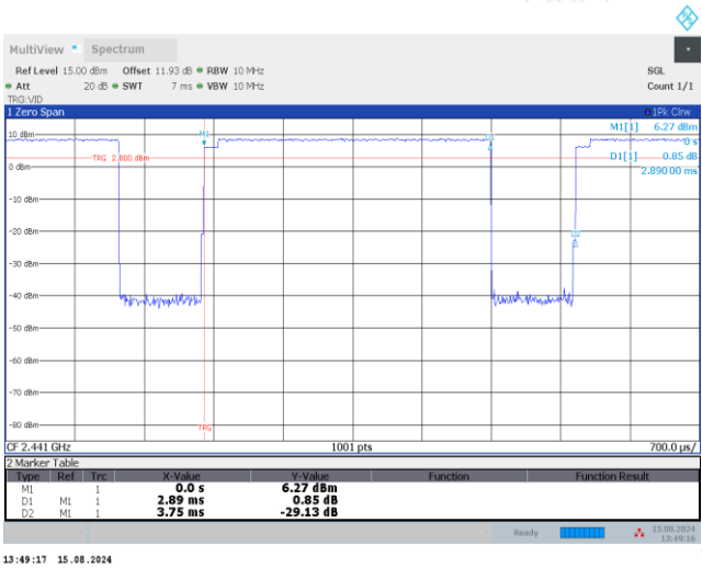
2DH5_2441MHz
