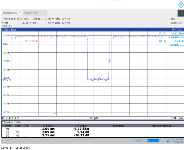
3DH5_2441MHz
