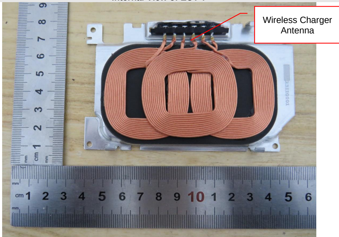
Internal View of EUT-8
