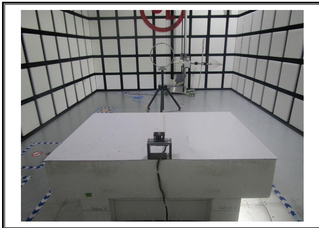
RADIATED EMISSIONS MEASUREMENT SETUP (Below 30MHz)
