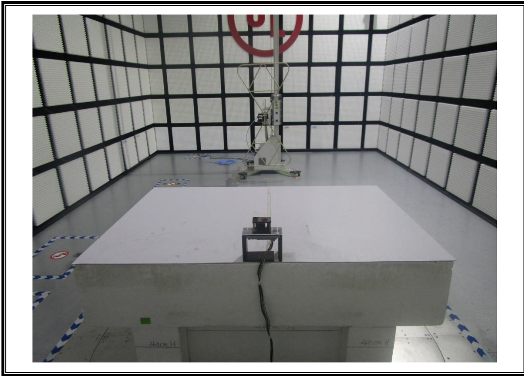
RADIATED EMISSIONS MEASUREMENT SETUP (30MHz ~ 1 GHz)
