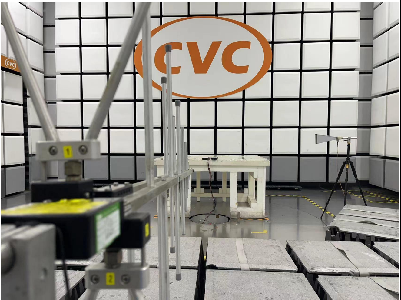
(1) Radiated spurious emission Test Setup(30MHz~1GHz)
