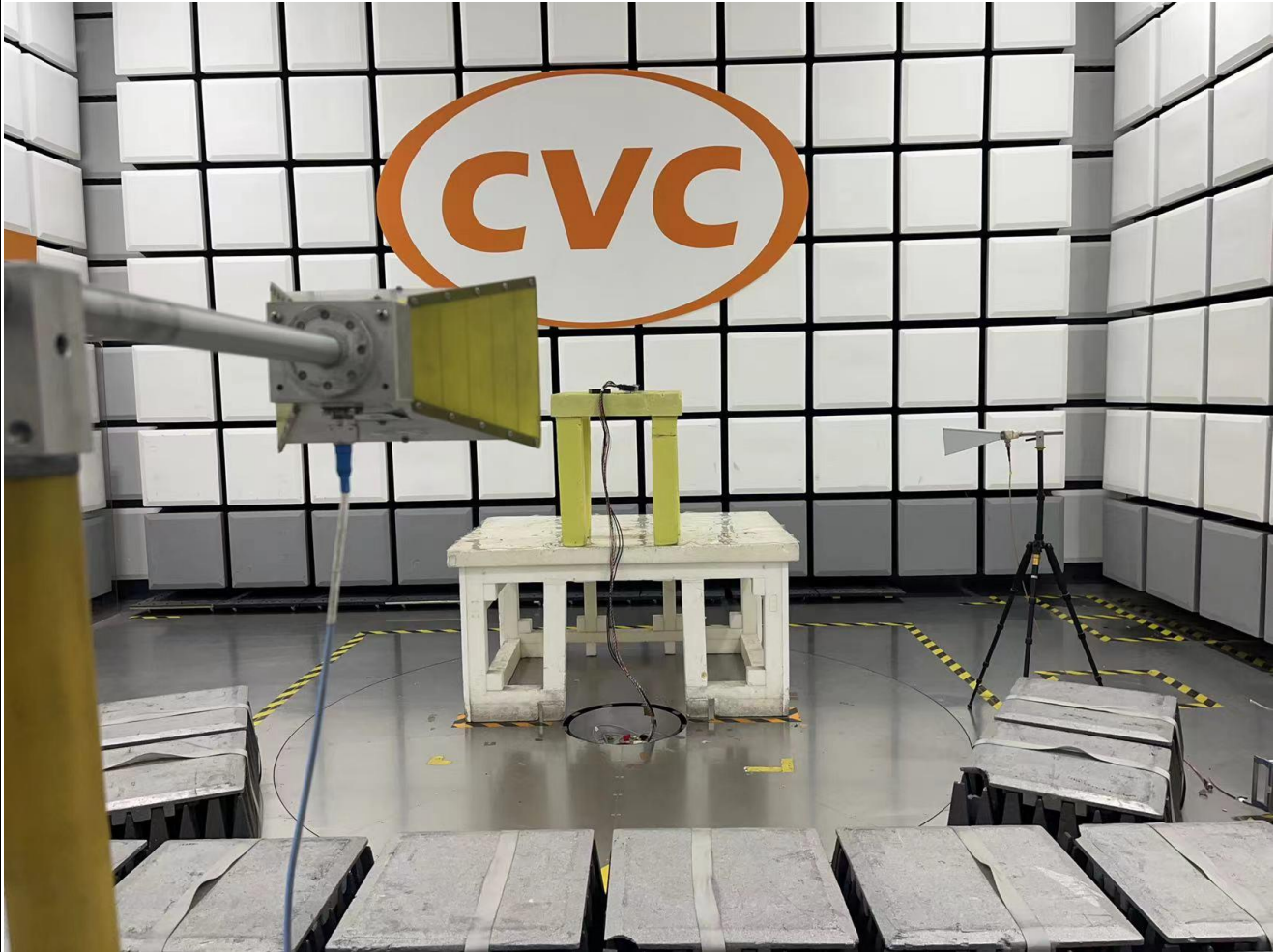
(2) Radiated spurious emission Test Setup(1GHz~18GHz)
