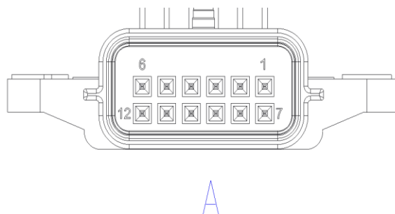
Figure 3 Interface Definition
