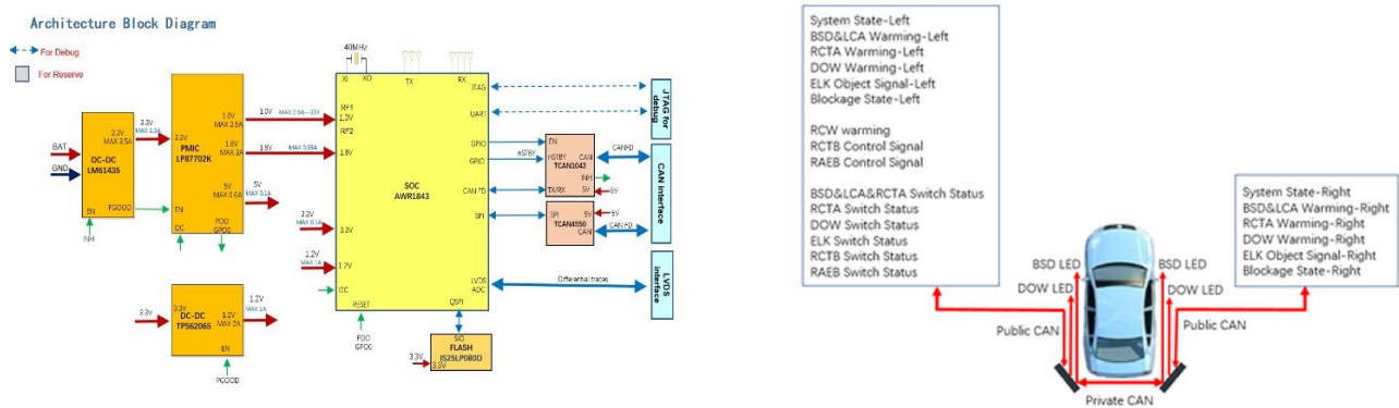
Figure 1 Block Diagram
