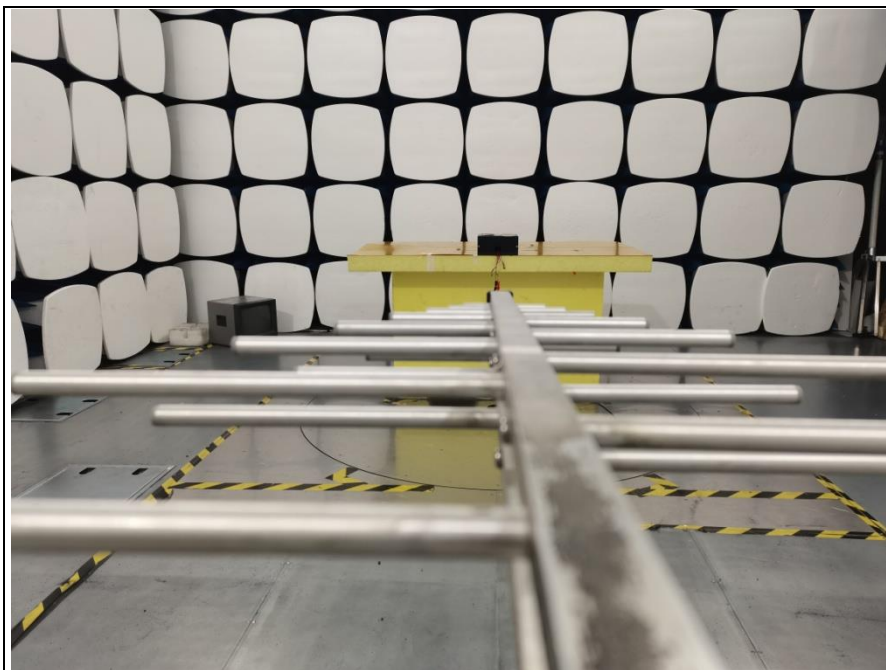
RADIATED EMISSIONS at frequencies up to 1 GHz-Mode 4
