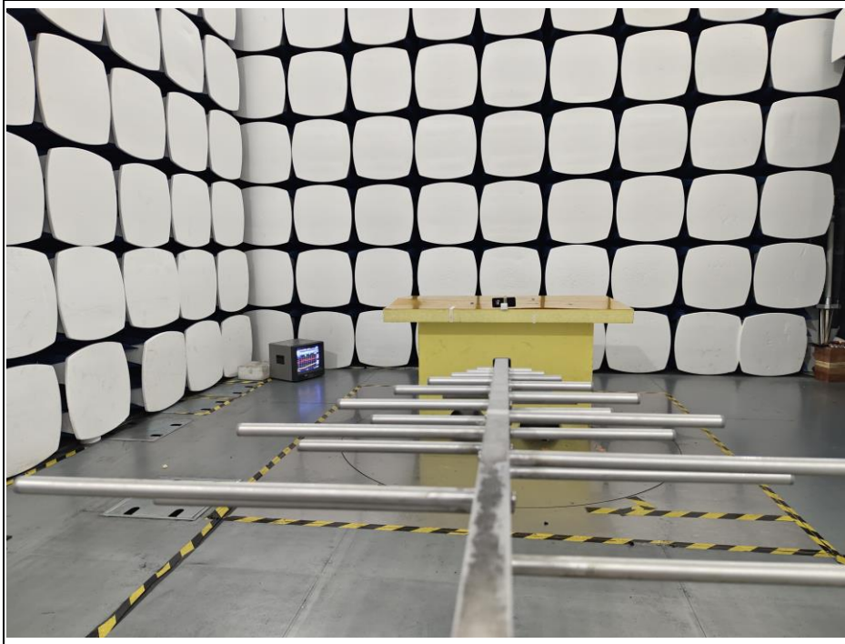
30MHz-1GHz
