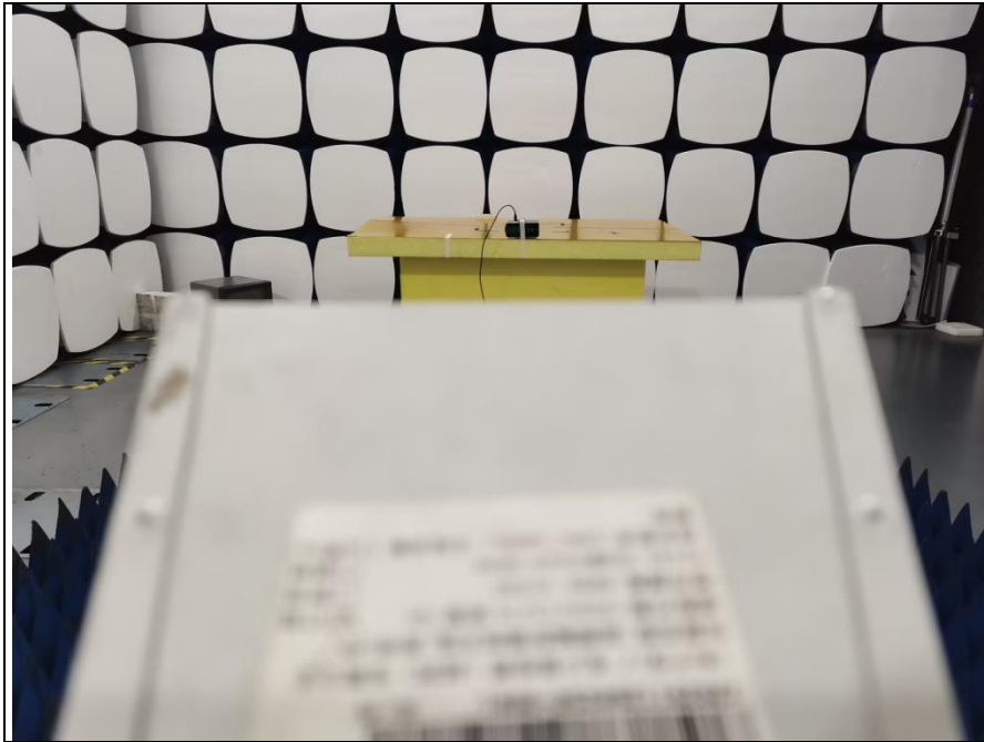
RADIATED EMISSIONS at frequencies above 1 GHz-Mode 1&2&3
