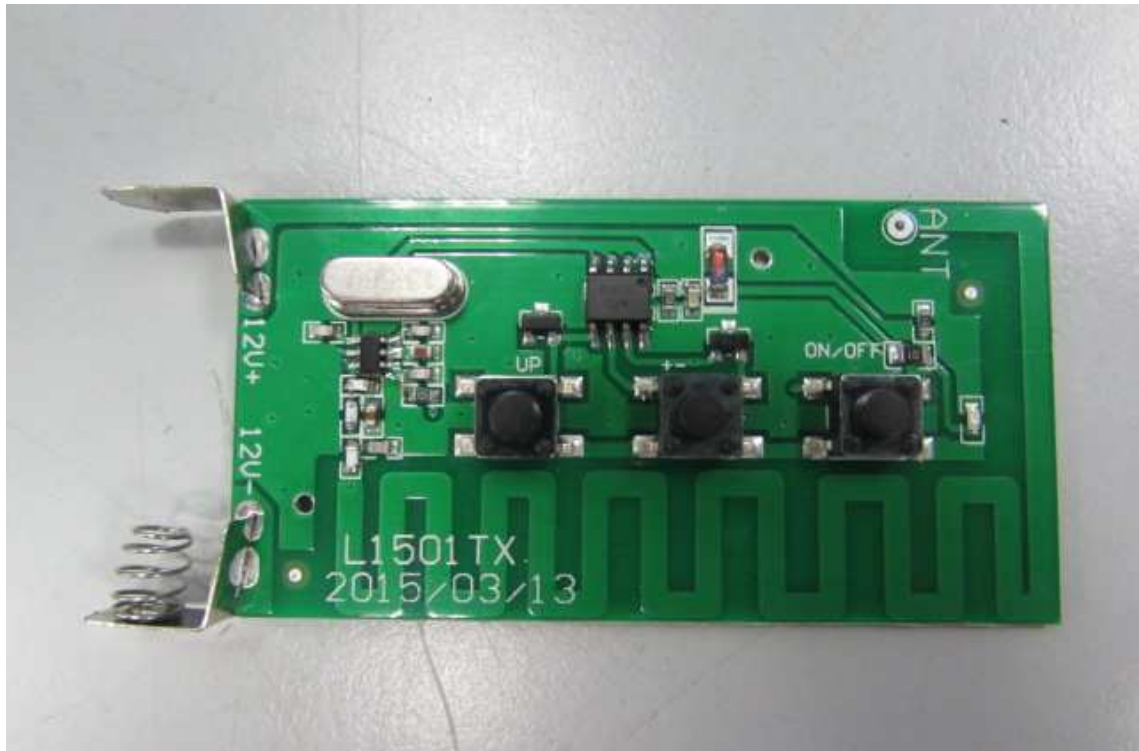
Main PCB view
