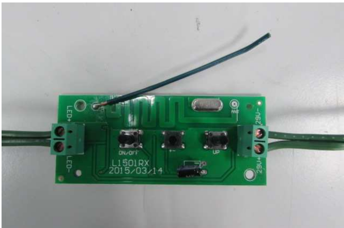
Receiver controller PCB view
