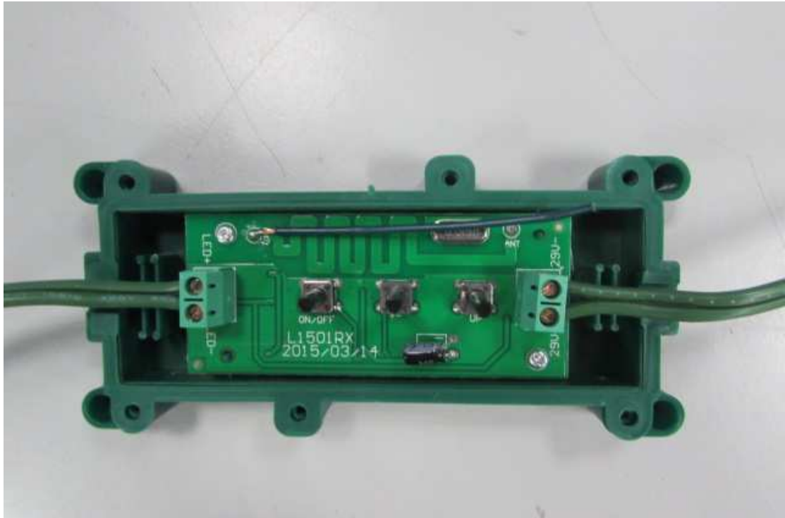
Receiver controller view
