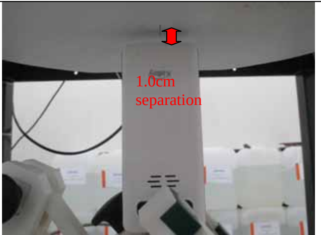
Body-Worn(Bottom edge)
