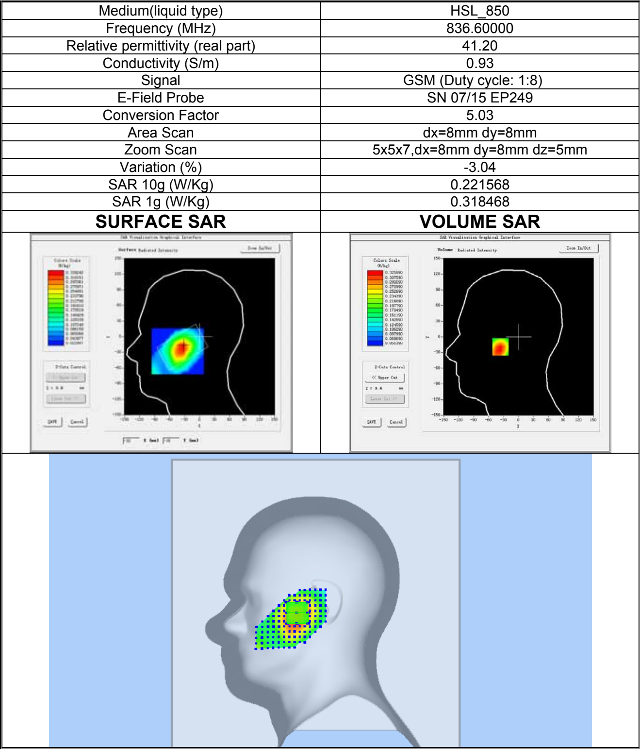
Plot 2: GSM850MHz, Mid channel (Right Head , Tilt) Product Description: Feature Phone Urban Test Date:2018-01-06
