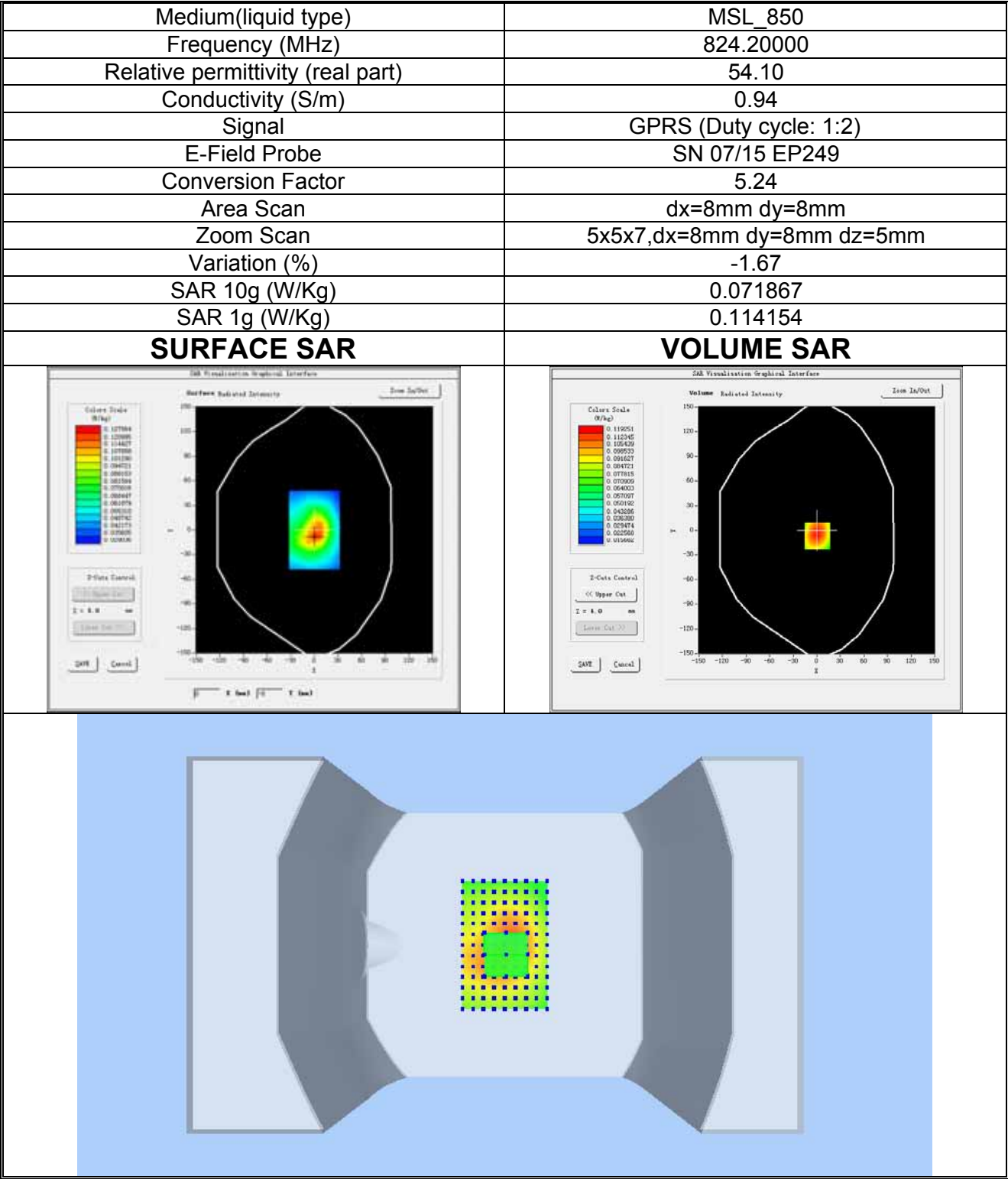
Plot 8: GPRS850MHz, Low channel(Body-worn, Bottom edge) Product Description: Feature Phone Urban Test Date: 2018-01-06
