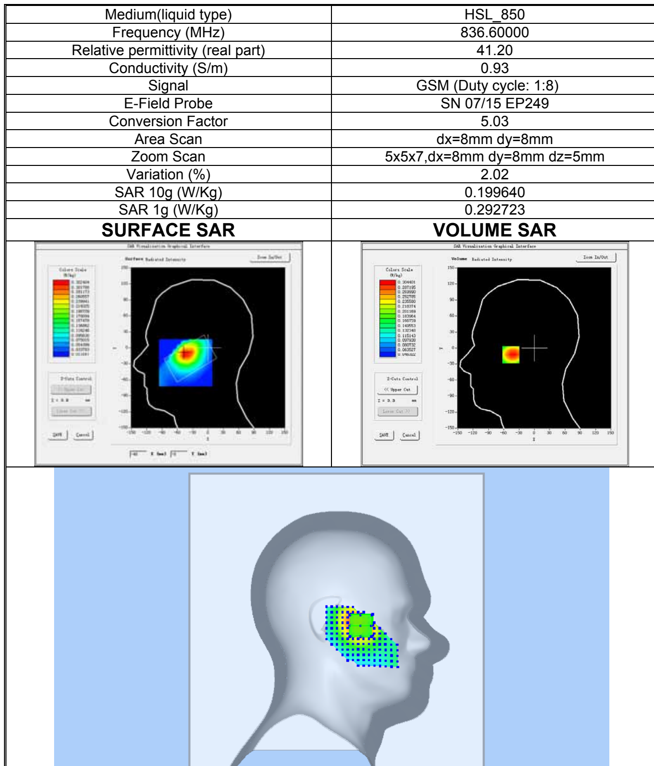
Plot 4: GSM850MHz, Mid channel (Left Head , Tilt) Product Description: Feature Phone Urban Test Date:2018-01-06
