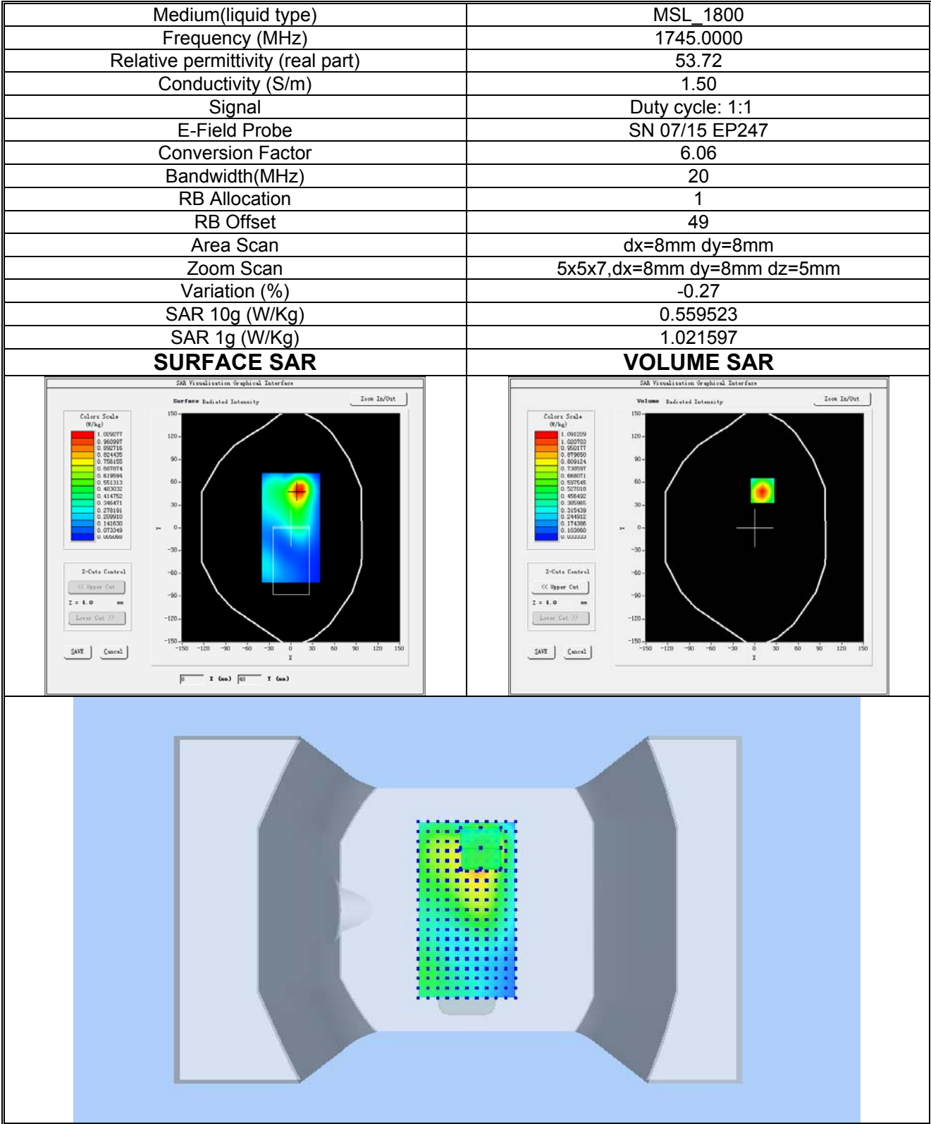
Plot 10:LTE BAND4, High channel (Body-worn/Hotspot, Back Surface) Product Description:Smart phone Test Date: 2019-06-27
