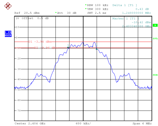
Mode: TX GFSK channel 1
