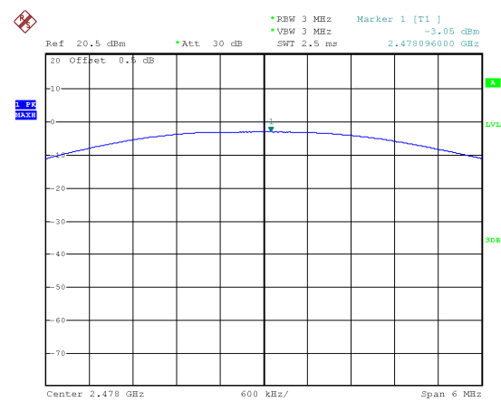
Mode: TX GFSK channel 38
