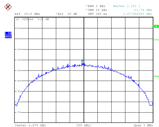
Mode: TX GFSK channel 38
