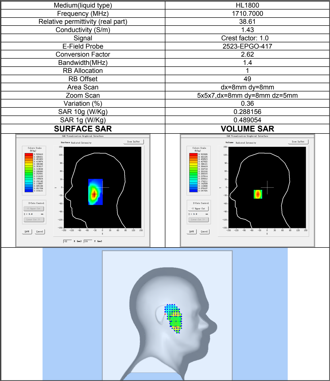
Plot 25:LTE BAND 66, Low channel (Left Head Cheek) Product Description: Smart Phone Test Date: 2025-07-12
