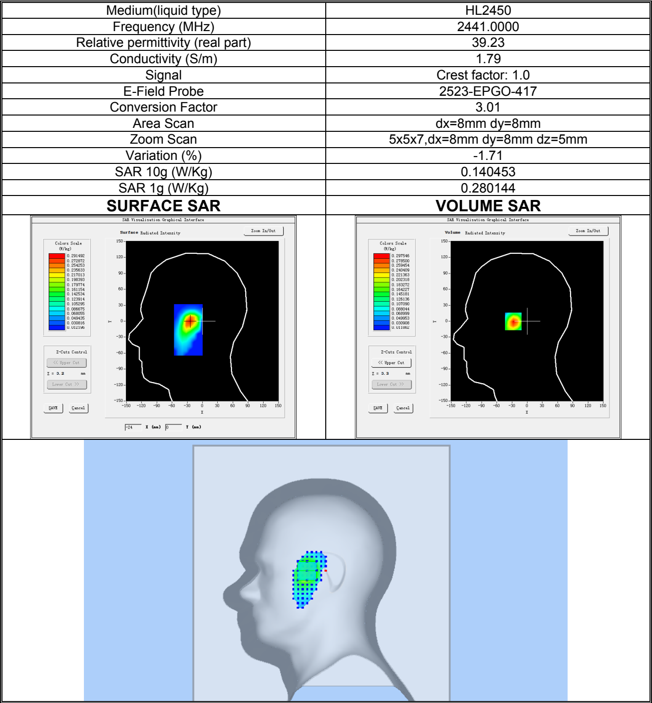
Plot 29: Bluetooth, Middle channel (Right Head Cheek) Product Description: Smart Phone Test Date: 2025-07-15
