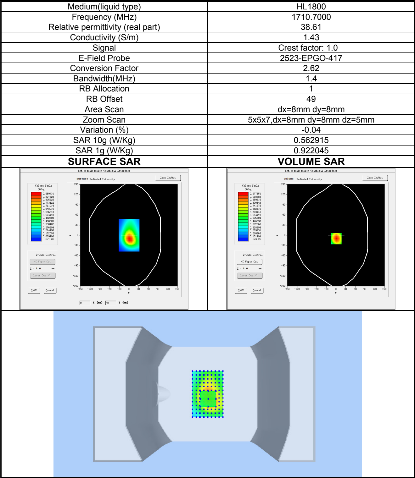
Plot 26: LTE BAND 66, Low channel (Body-worn/ Hotspot, Back Side) Product Description: Smart Phone Test Date: 2025-07-12
