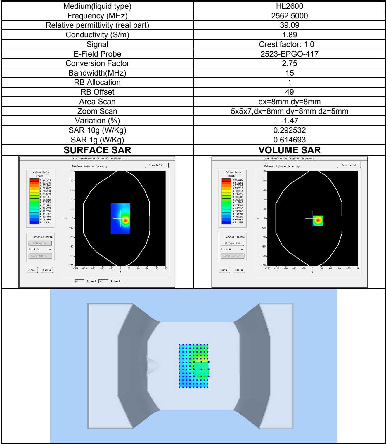
Plot 18: LTE BAND 7, High channel (Body-worn/ Hotspot, Back Side) Product Description: Smart Phone Test Date: 2025-07-15
