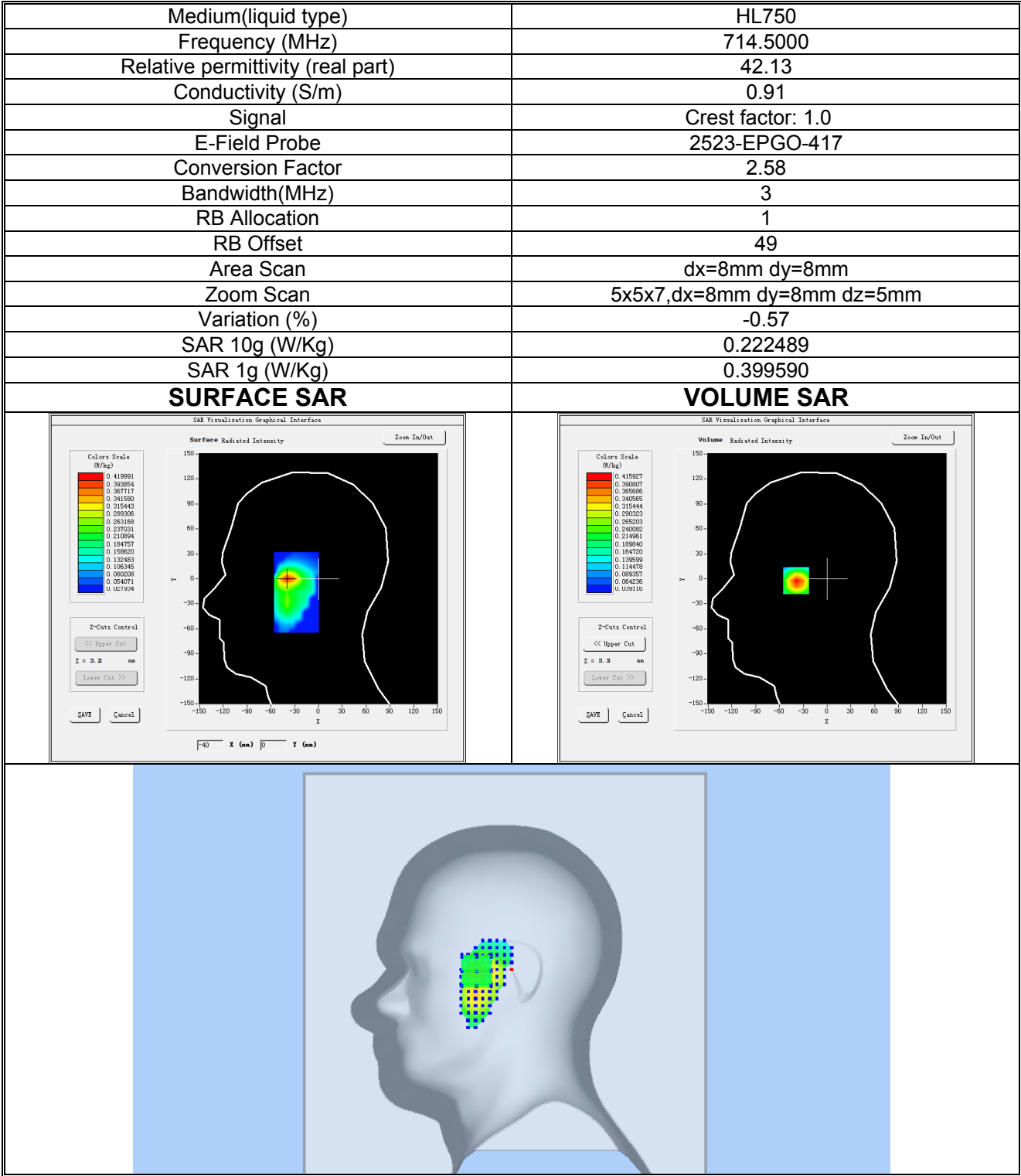
Plot 19:LTE BAND 12, High channel (Right Head Cheek) Product Description: Smart Phone Test Date: 2025-07-16
