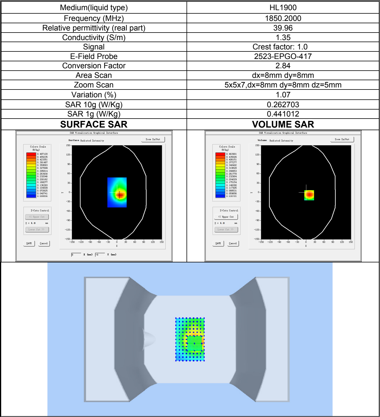
Plot 4: GSM 1900, Low channel (Body-worn /Hotspot, Back Side) Product Description: Smart Phone Test Date: 2025-07-14
