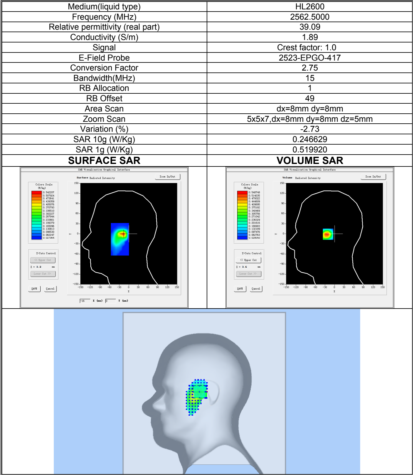
Plot 17:LTE BAND 7, High channel (Right Head Cheek) Product Description: Smart Phone Test Date: 2025-07-15
