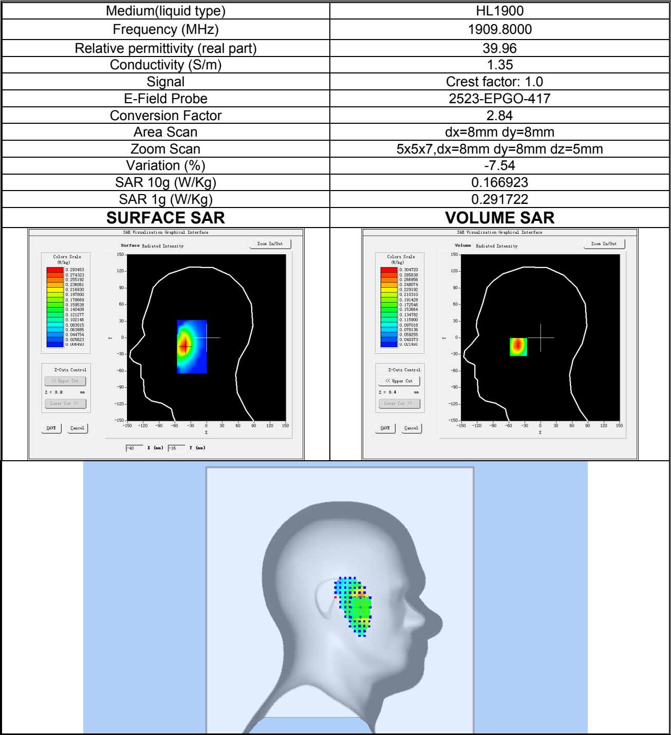
Plot 3: GSM 1900, High channel (Left Head Cheek) Product Description: Smart Phone Test Date: 2025-07-14
