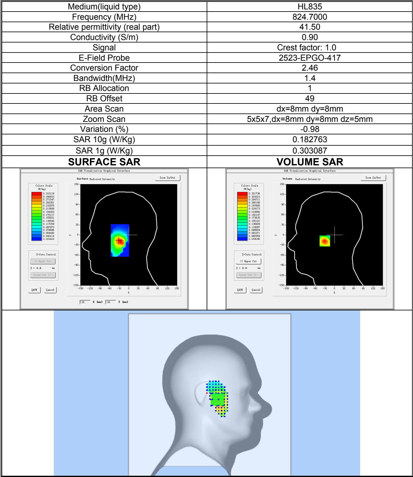
Plot 15:LTE BAND 5, Low channel (Left Head Cheek) Product Description: Smart Phone Test Date: 2025-07-16
