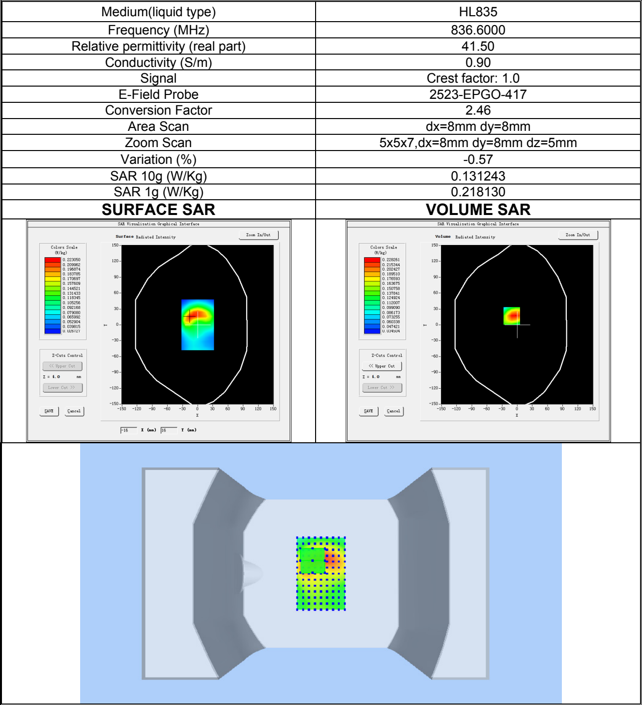
Plot 10: WCDMA BAND V, Middle channel (Body-worn/Hotspot, Back Side) Product Description: Smart Phone Test Date: 2025-07-16
