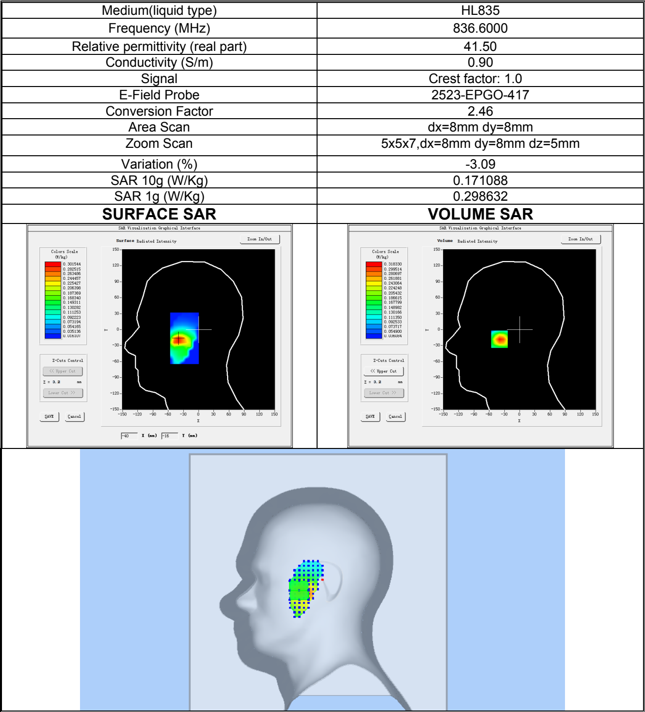
Plot 9: WCDMA BAND V, Middle channel (Right Head Cheek) Product Description: Smart Phone Test Date: 2025-07-16
