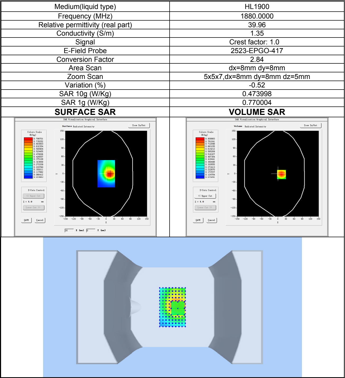
Plot 6: WCDMA BAND II, Middle channel (Body-worn /Hotspot, Back Side) Product Description: Smart Phone Test Date: 2025-07-14
