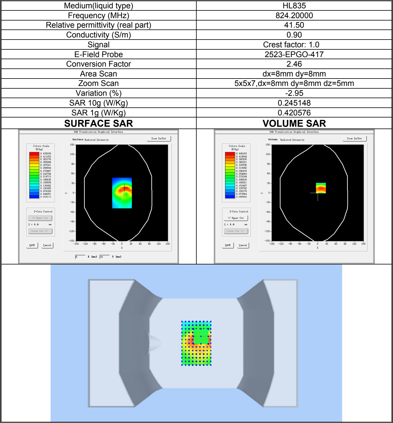
Plot 2: GPRS850, Low channel (Body-worn /Hotspot, Back Side) Product Description:Smart Phone Test Date: 2025-07-16
