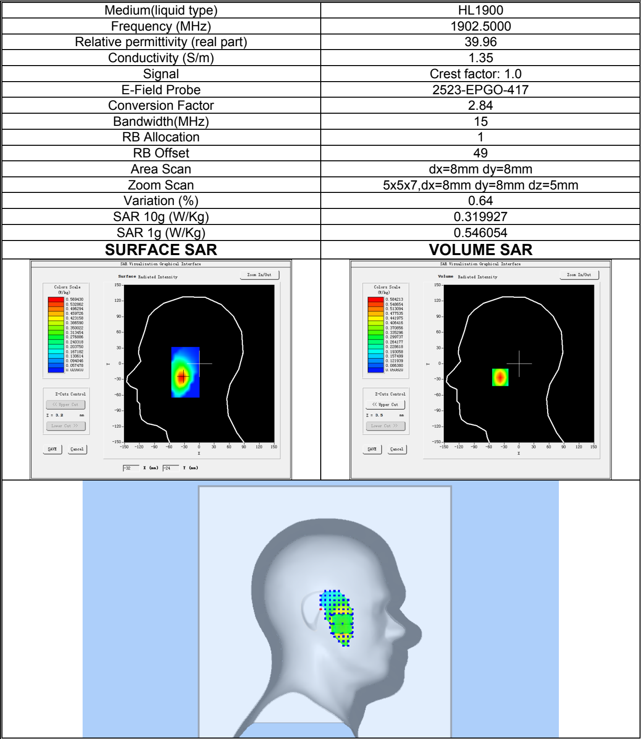
Plot 11:LTE BAND 2, High channel (Left Head Cheek) Product Description:Smart Phone Test Date: 2025-07-14
