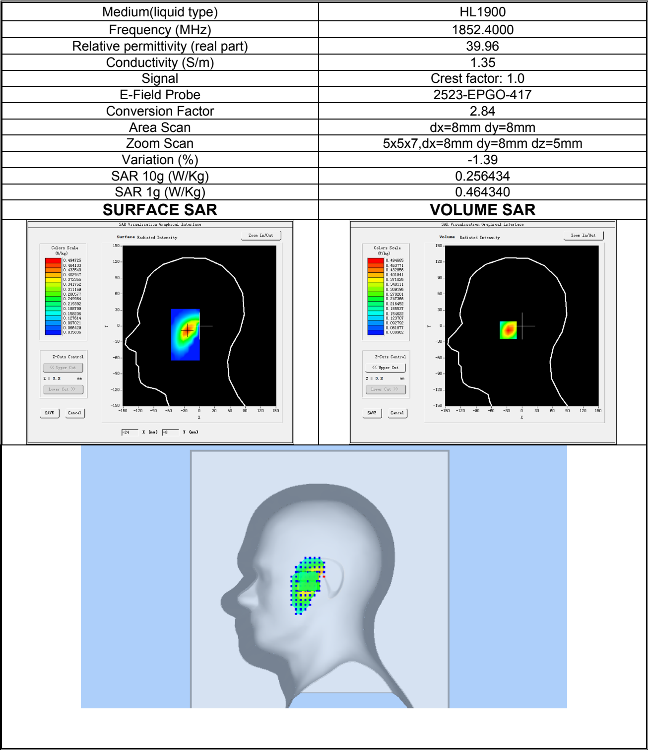
Plot 5: WCDMA BAND II, Low channel (Right Head Cheek) Product Description: Smart Phone Test Date: 2025-07-14
