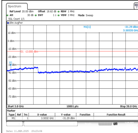
Band4-3MHz-QPSK-20385-1RB#0-3000~20000-
