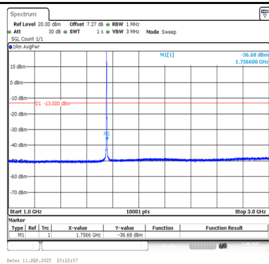
Band4-3MHz-QPSK-20385-1RB#0-1000~3000-PA
