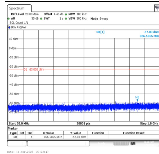
Band4-3MHz-QPSK-20385-1RB#0-30~1000-PAS
