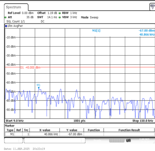
Band4-3MHz-16QAM-20385-1RB#0-0.009~0.15-P
