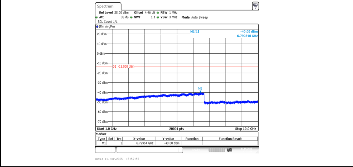
Band5-4233-5-1000~10000MHz-PASS
