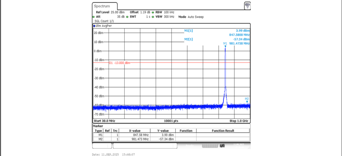
Band5-4233-3-30~1000MHz-PASS
