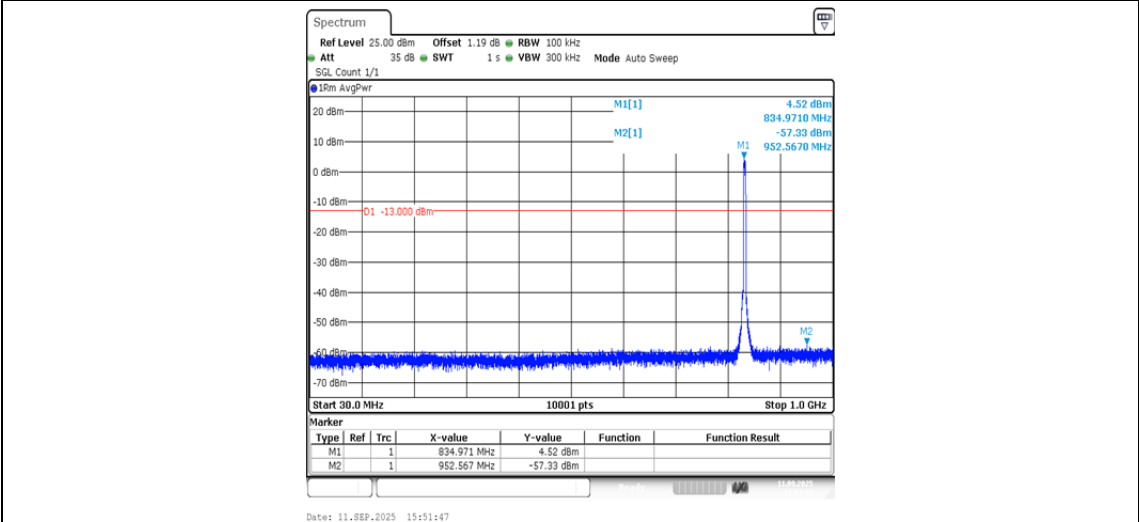
Band5-4182-5-30~1000MHz-PASS
