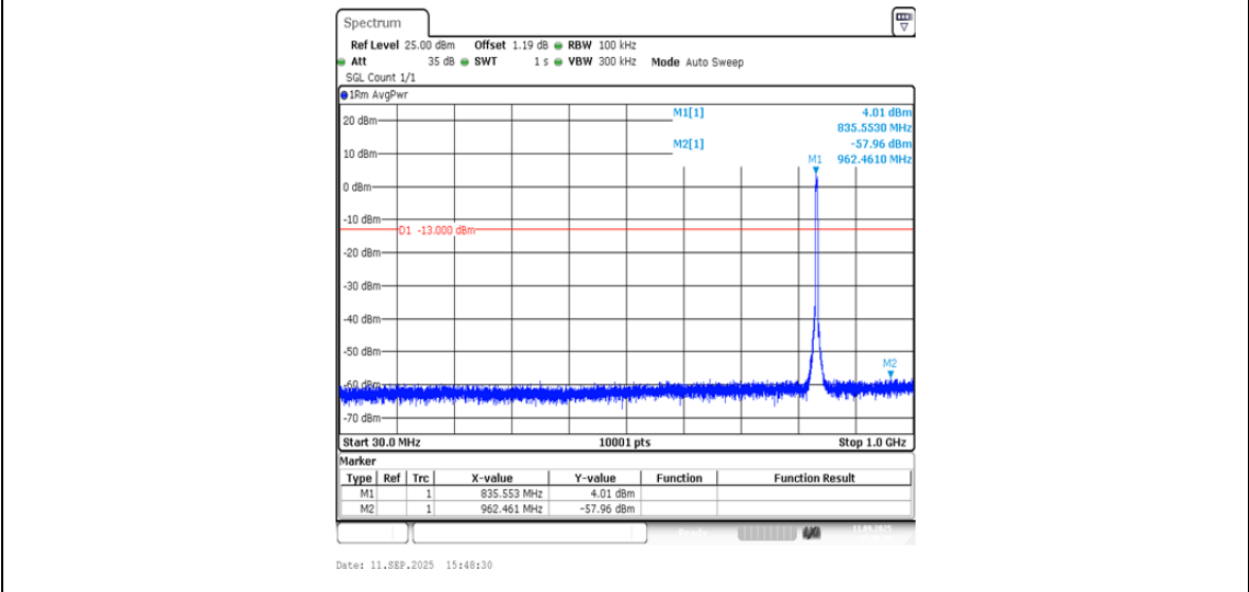
Band5-4182-4-30~1000MHz-PASS
