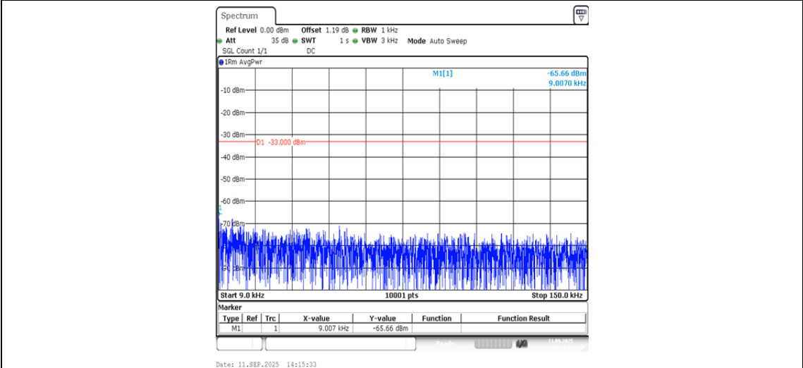
Band5-4233-0.009~0.15MHz-PASS
