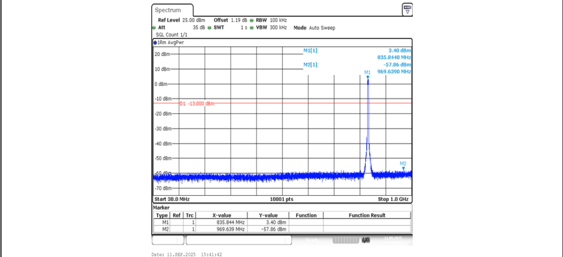
Band5-4182-2-30~1000MHz-PASS
