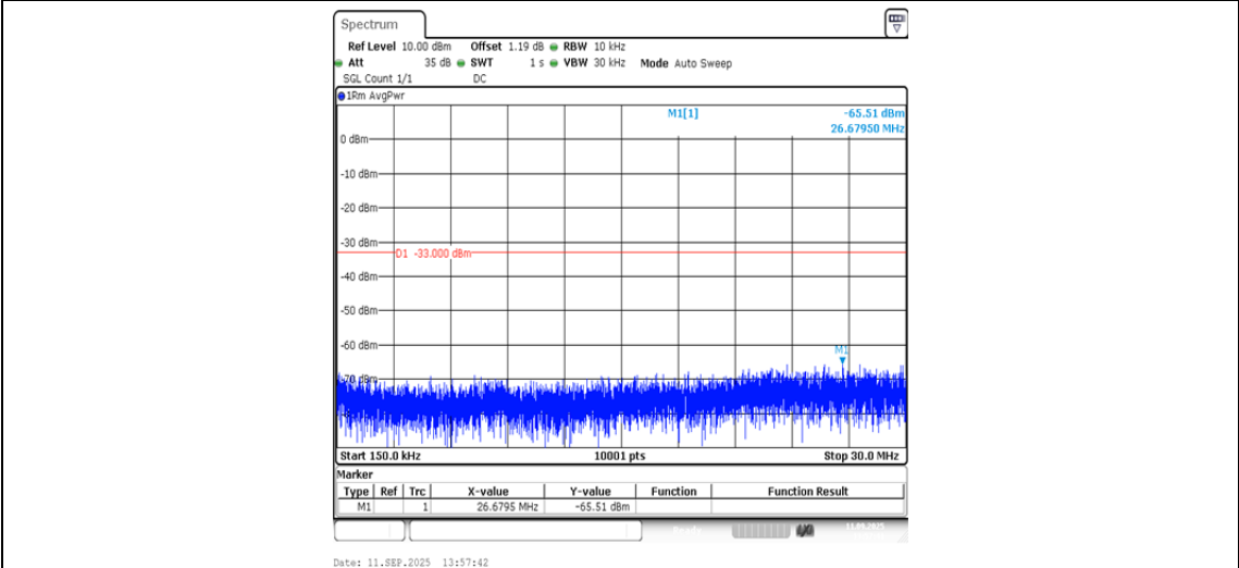
Band4-1312-3-0.15~30MHz-PASS
