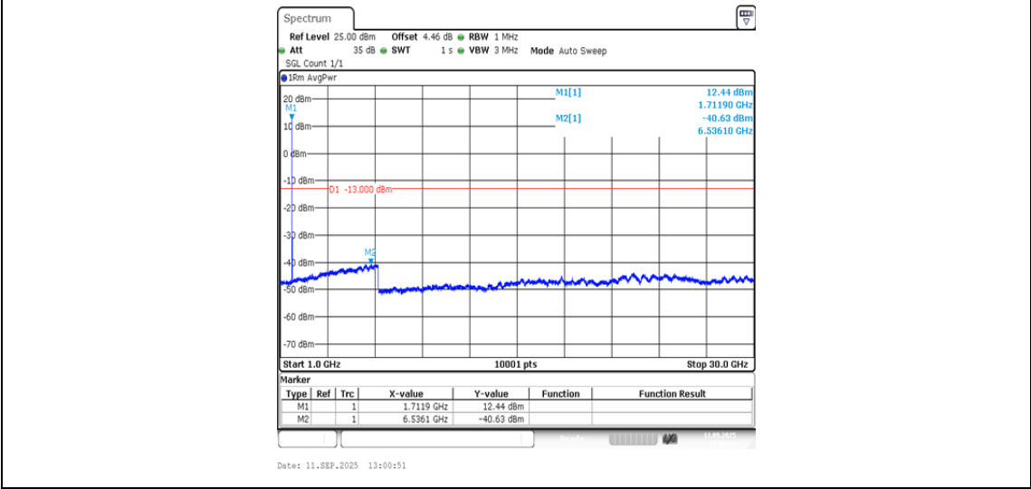
Band4-1312-2-1000~30000MHz-PASS
