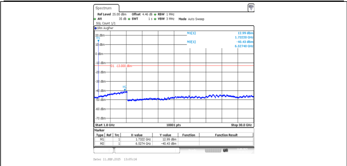
Band4-1413-3-1000~30000MHz-PASS
