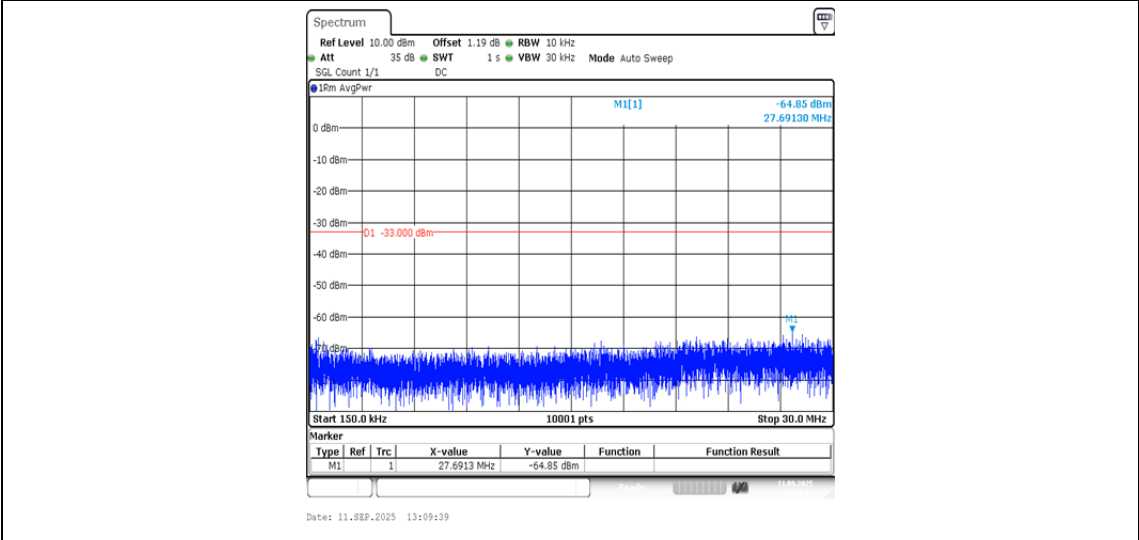
Band4-1513-4-0.15~30MHz-PASS
