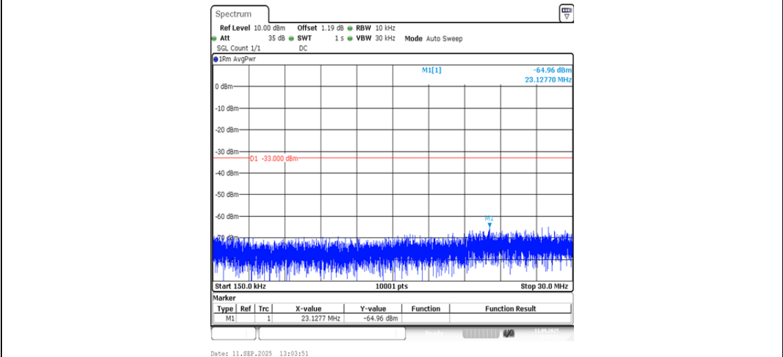
Band4-1312-3-0.15~30MHz-PASS
