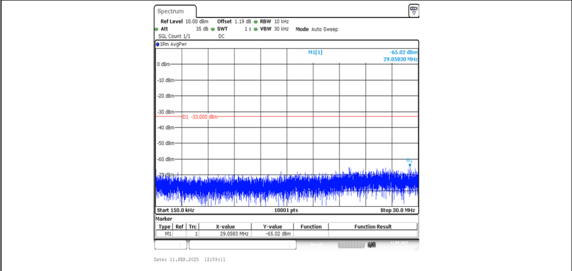
Band4-1513-1-0.15~30MHz-PASS
