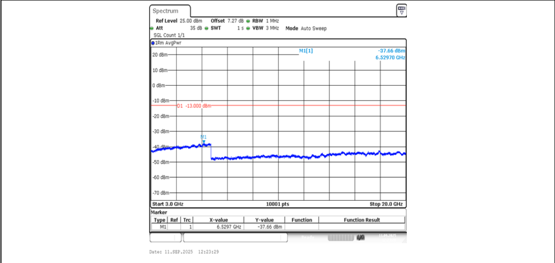
Band2-9538-5-3000~20000MHz-PASS
