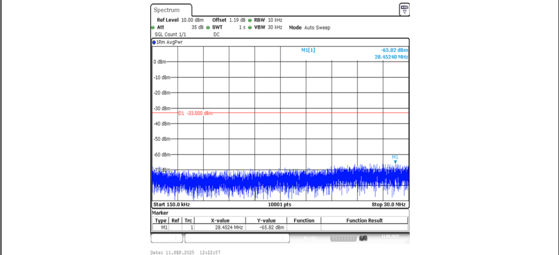
Band2-9538-5-0.15~30MHz-PASS
