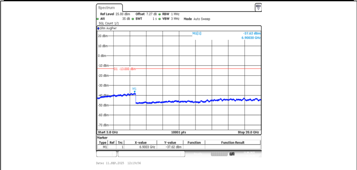
Band2-9538-4-3000~20000MHz-PASS
