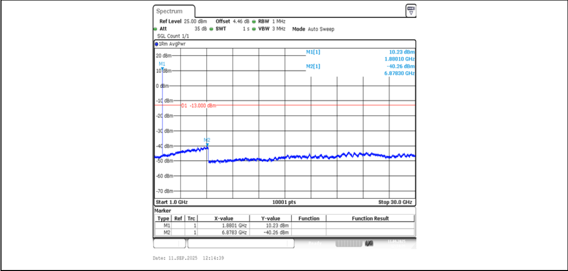
Band2-9400-3-1000~30000MHz-PASS
