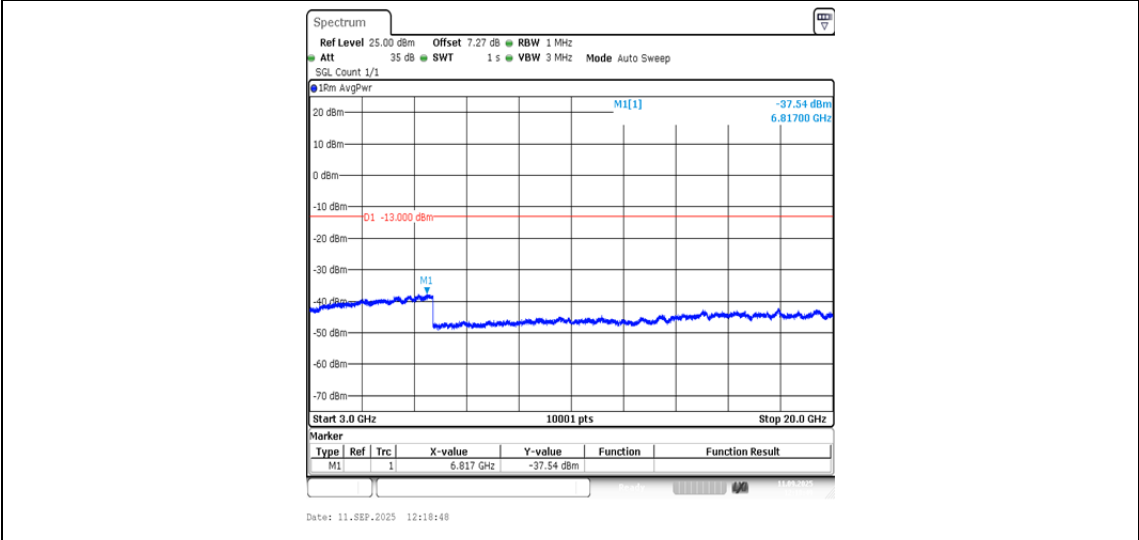
Band2-9400-4-3000~20000MHz-PASS
