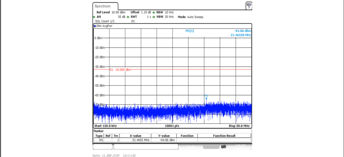
Band2-9538-2-0.15~30MHz-PASS
