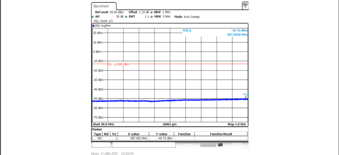
Band2-9400-5-30~1000MHz-PASS
